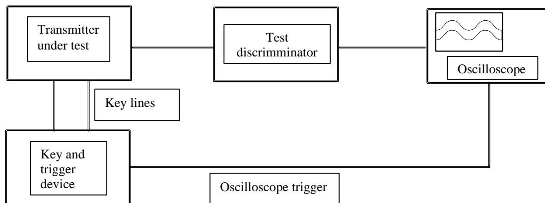
Figure 3: Measurement arrangement
