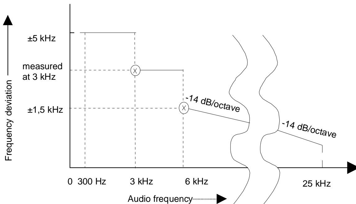
Figure 1: Frequency deviation
