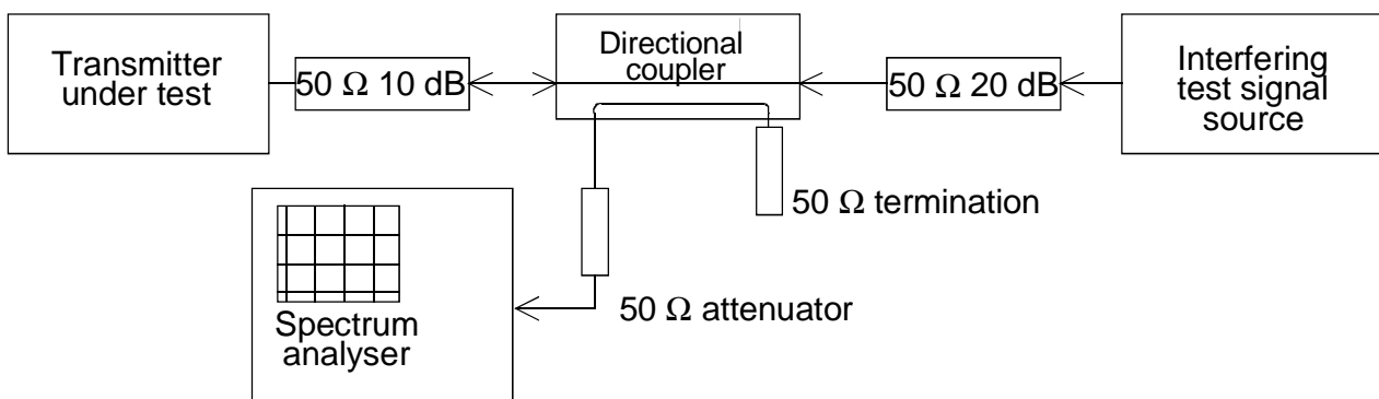
Figure 7: Measurement arrangement
