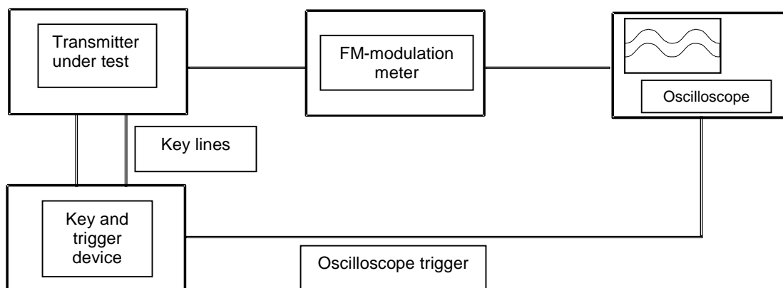
Figure 3: Measurement arrangement
