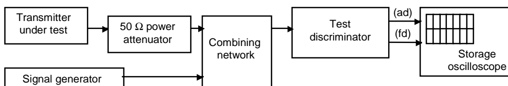
Figure 5: Measurement arrangement
