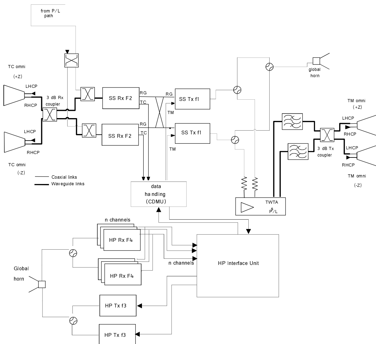
Figure A.6: Baseline Configuration typical TCR/RF architecture
