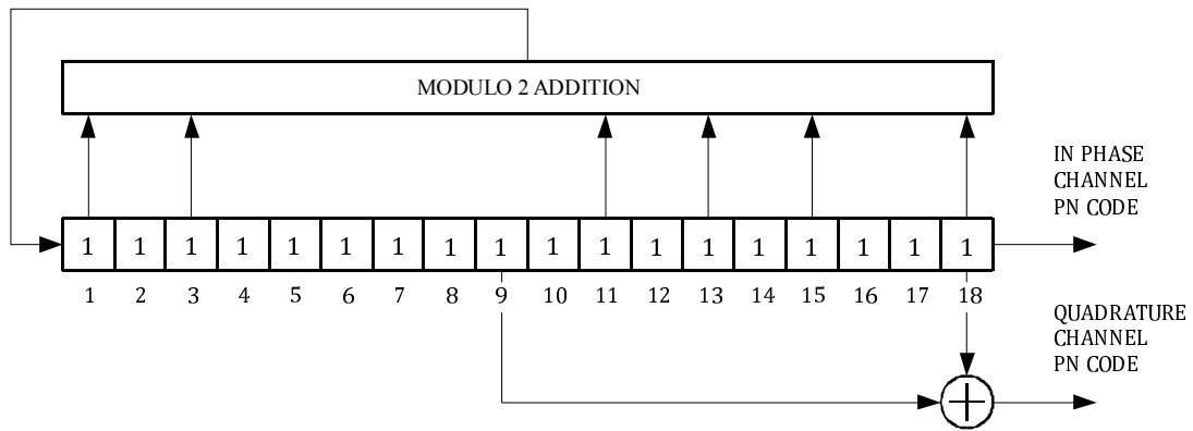
Figure E.8: Example of tap connections for maximum length code based on code set 1, MTC2 (table E.5), used for MTC3-tracking, in-phase and quadrature-phase channel. Quadrature-phase channel is also transmitted for acquisition.
