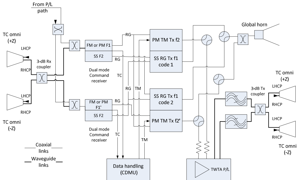
Figure A.5: Configuration 3 typical TCR/RF architecture
