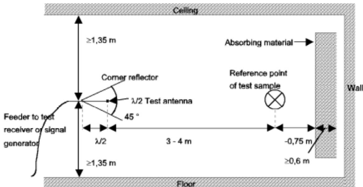
Figure C.2: Indoor site arrangement (shown for horizontal polarization)
