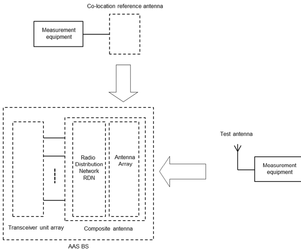
Figure D.4: Receiver test interfaces for co-location concept
