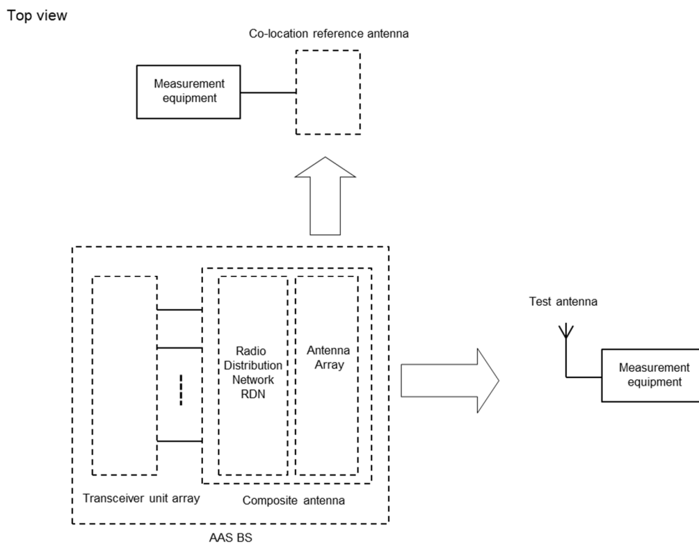
Figure D.2: Transmitter test interfaces for co-location concept
