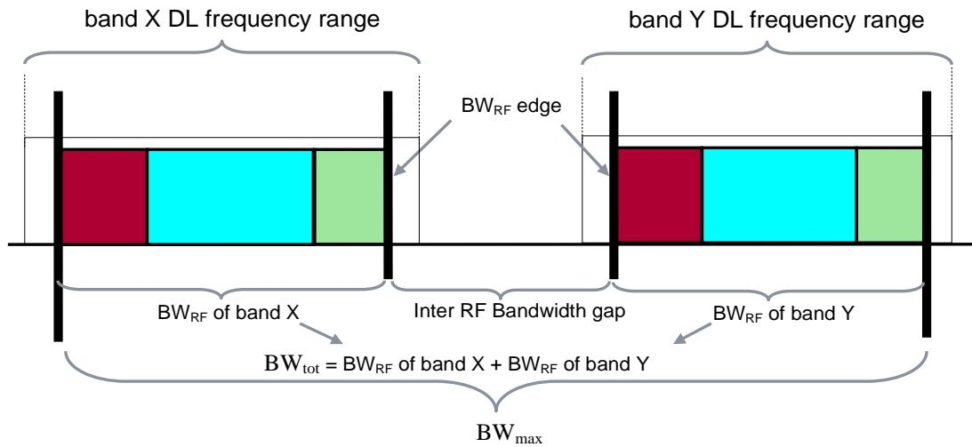
Figure 3.1-4: Maximum Radio Bandwidth BW_{max} and Total RF Bandwidth BW_{tot} for multi-band Base Station
