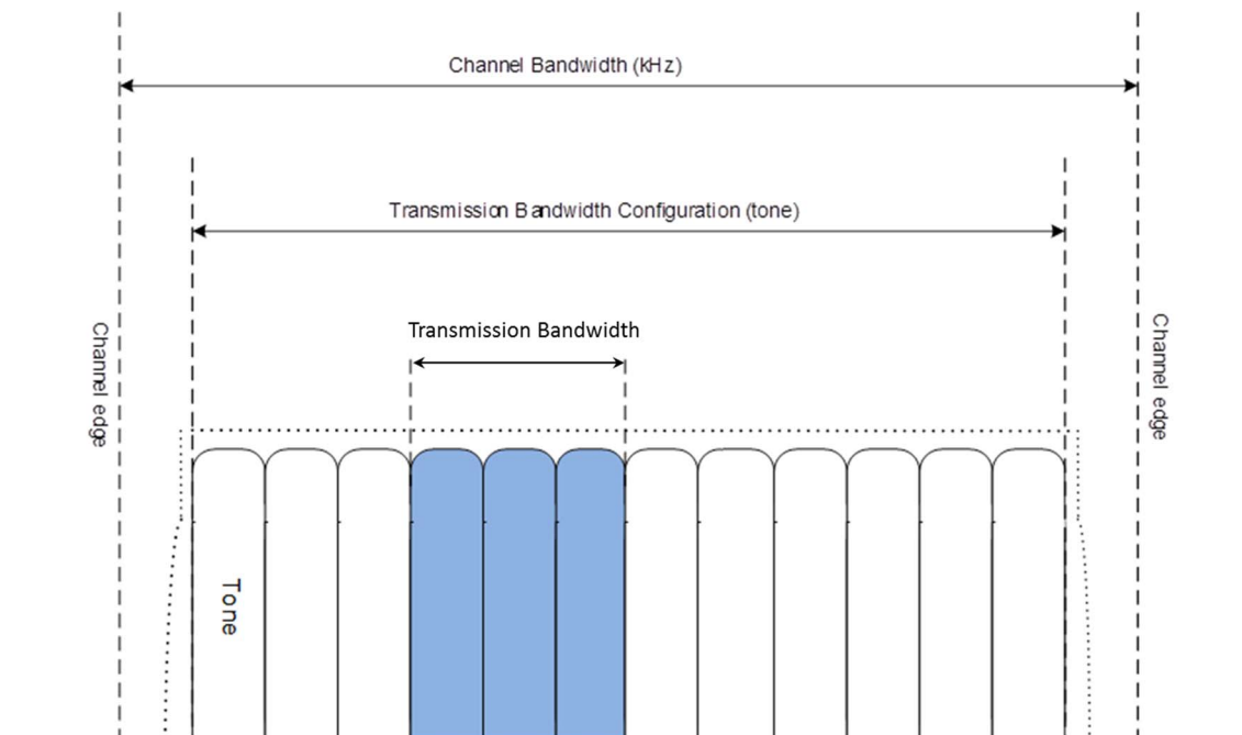
Figure 3.1-3: Definition of Channel Bandwidth and Transmission Bandwidth configuration for category NB1
