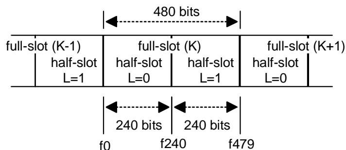
Figure 3: Half-slot format
