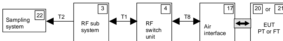
Figure 19: Test setup 1
