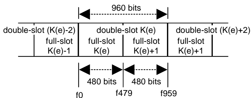
Figure 4: Double-slot format
