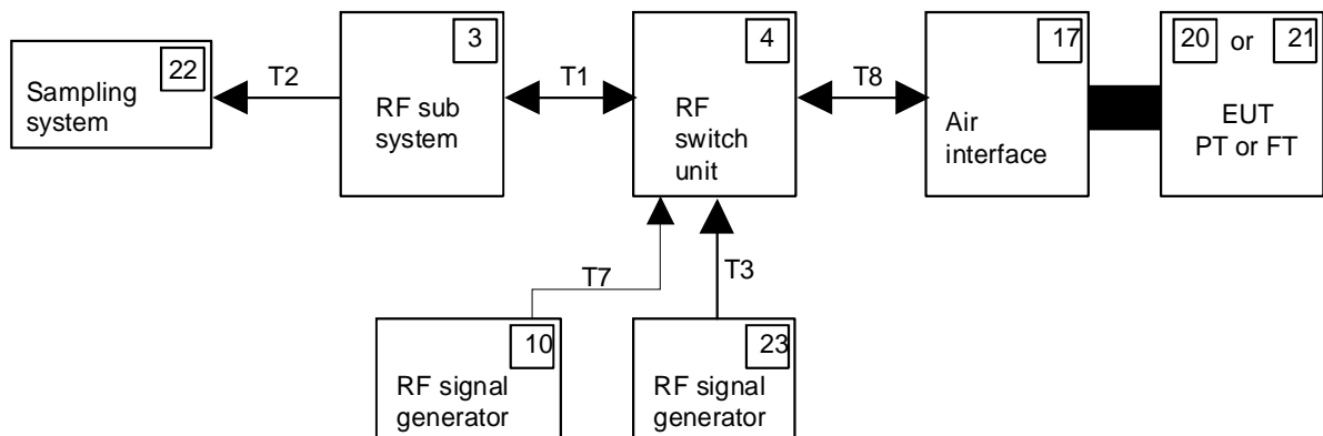
Figure 21: Test setup 3
