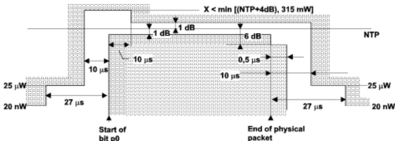
Figure 35: Power-time template
