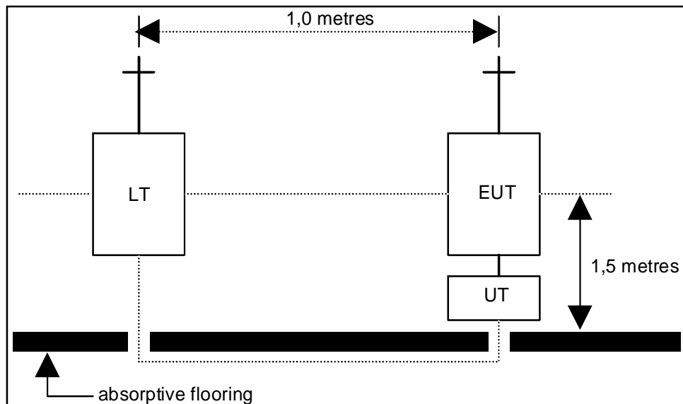
Figure 25: Testing arrangement
