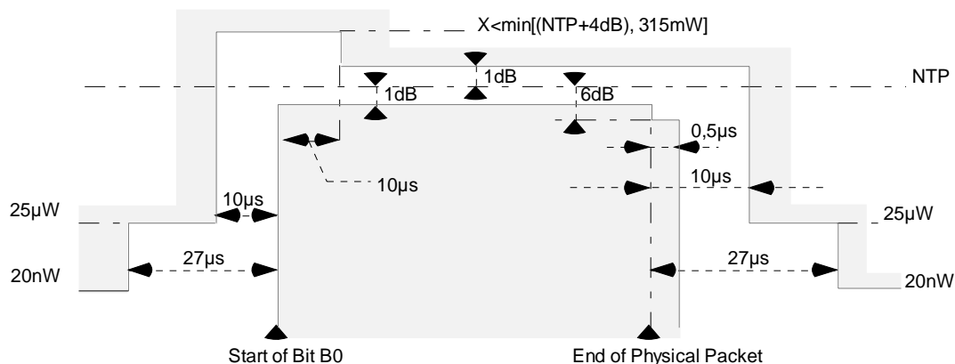
Figure 5: Physical packet power-time template [B0 shall be p0]
