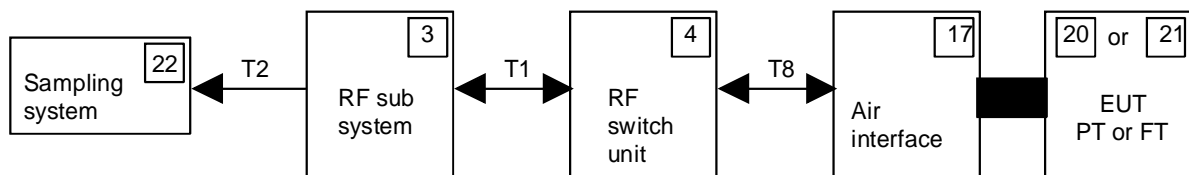
Figure 19: Test setup 1
