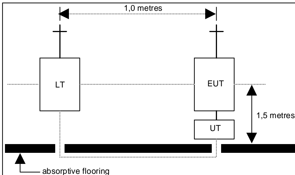
Figure 26: Testing arrangement
