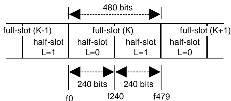
Figure 3: Half-slot format
