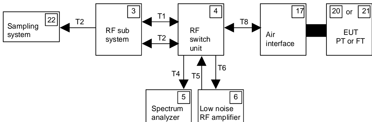
Figure 22: Test setup 4
