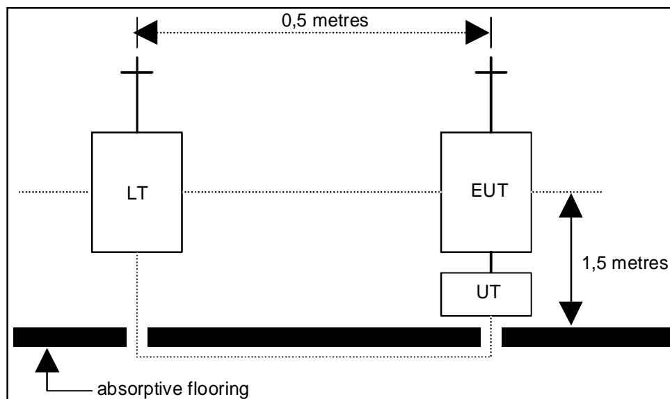
Figure 24: Testing arrangement
