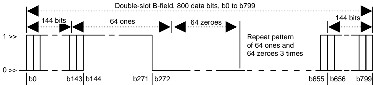
Figure 39: Test packet transmission for case 2, double-slot
