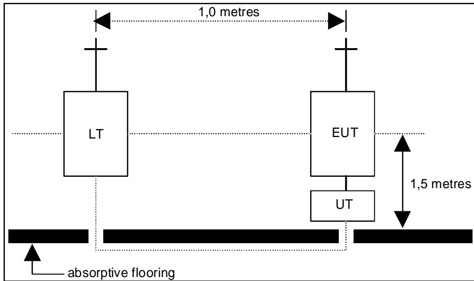
Figure 25: Testing arrangement
