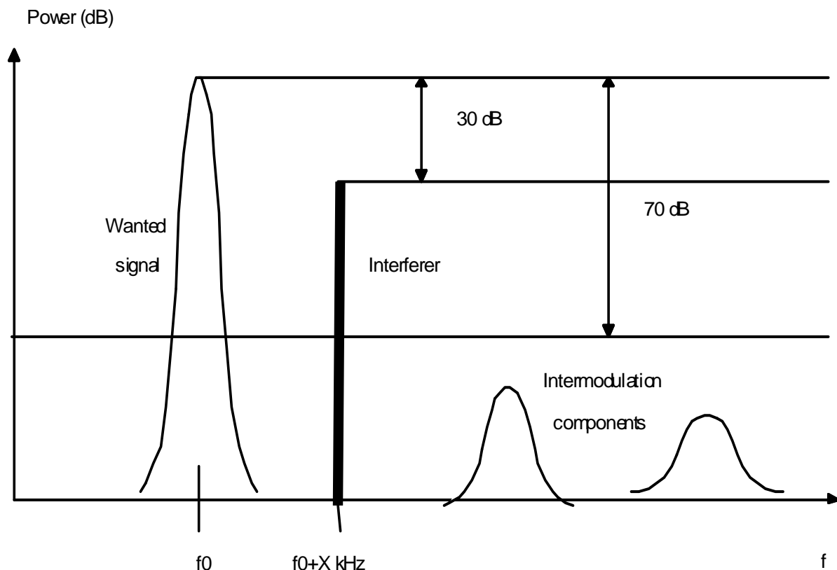
Figure 8: Example of TX intermodulation attenuation
