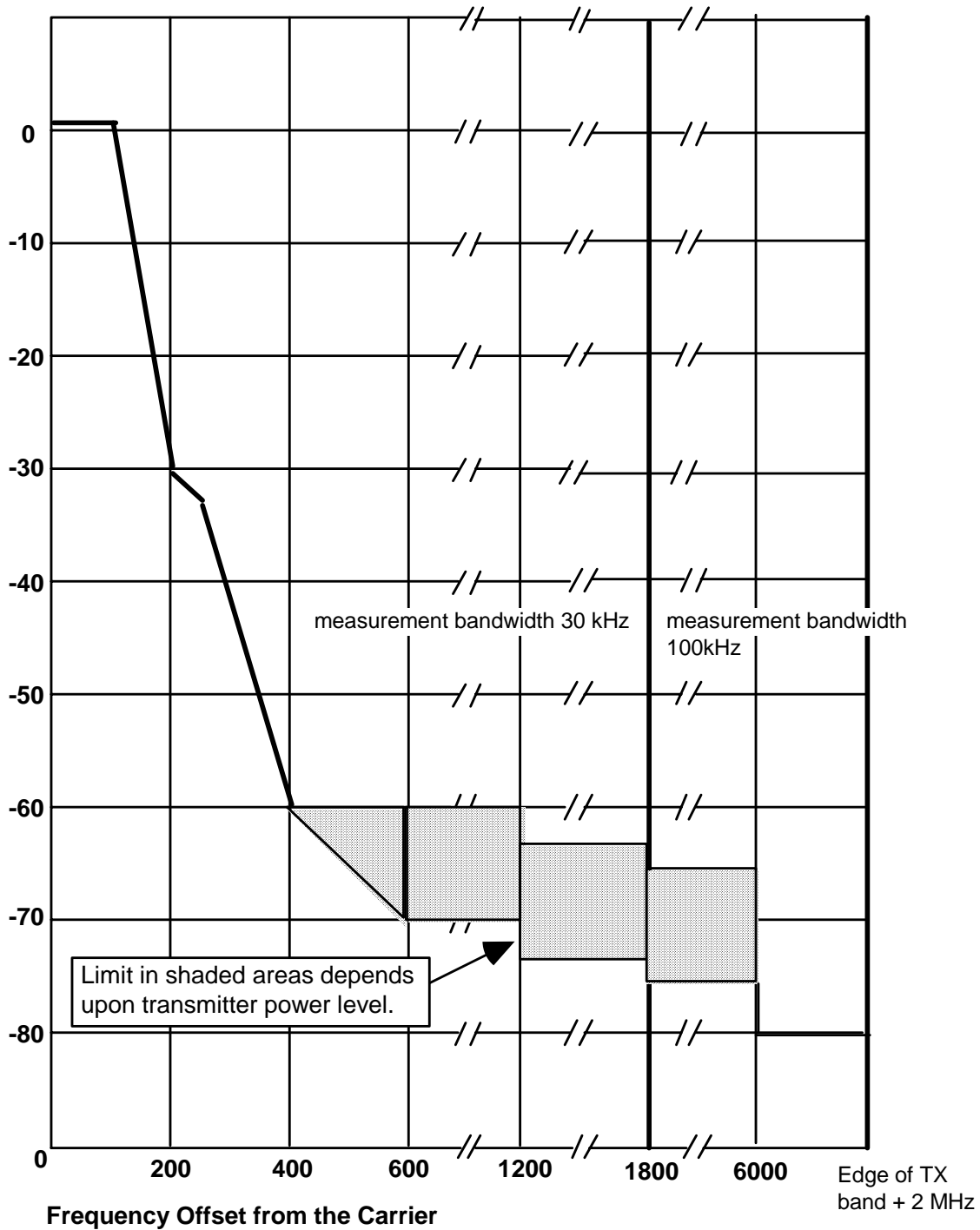
Figure 2: BTS Modulation and Noise Spectrum Mask due to GMSK modulation
