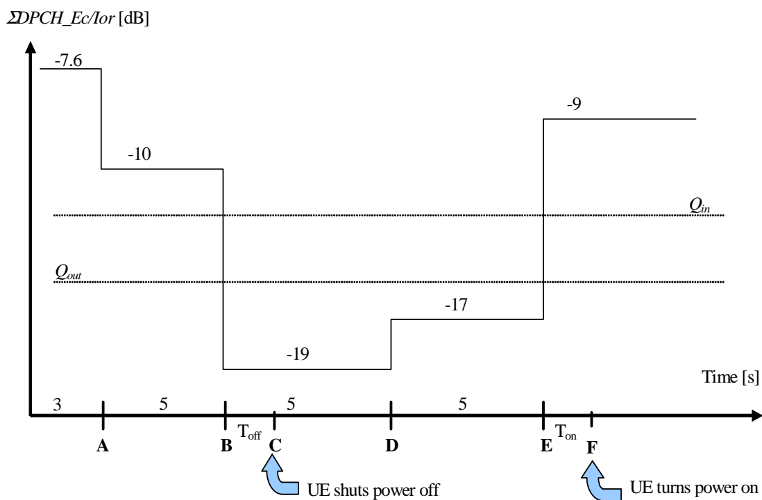
Figure 4.2.11.2.3-1: Test case for out-of-synchronization handling in the UE (7,68 Mcps TDD option)
