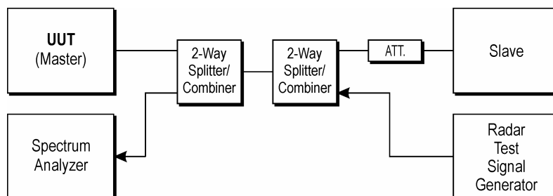
Figure 4: Set-up where UUT is a Master and radar test signals are injected into the Master
