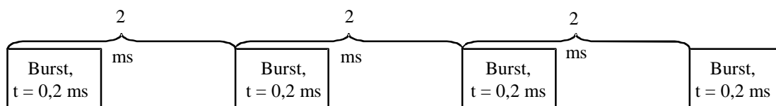
Figure 3: General structure of the test transmission sequences
