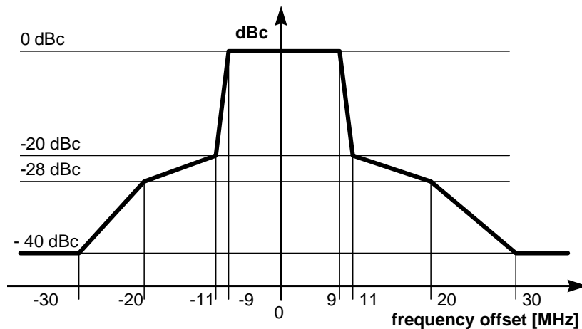
Figure 2: Transmit spectral power mask. dBc is the spectral density relative to the maximum spectral power density of the transmitted signal.
