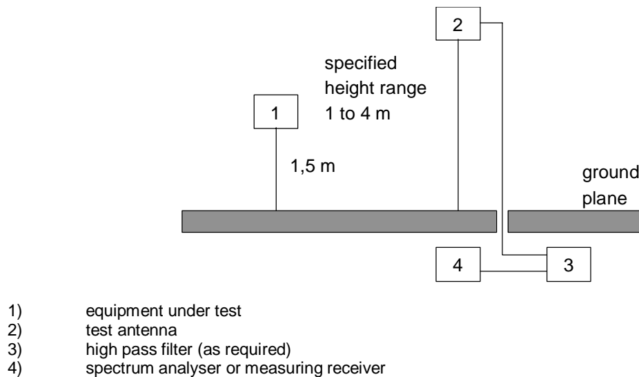
Figure B.1: Measuring arrangement
