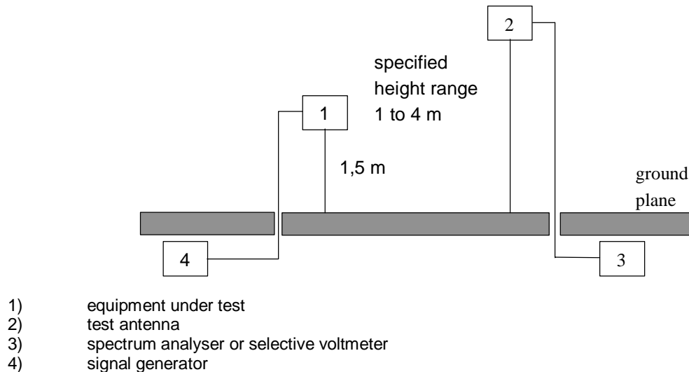
Figure C.2: Measurement arrangement N82
