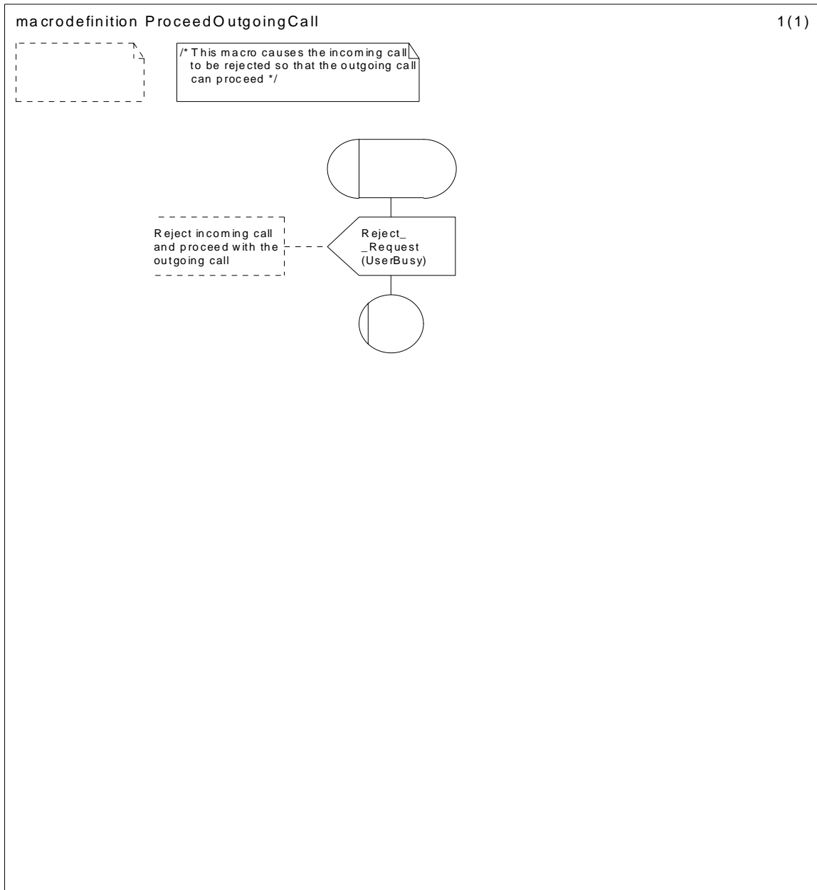
Figure C.2: SDL macro definition ProceedOutgoingCall
