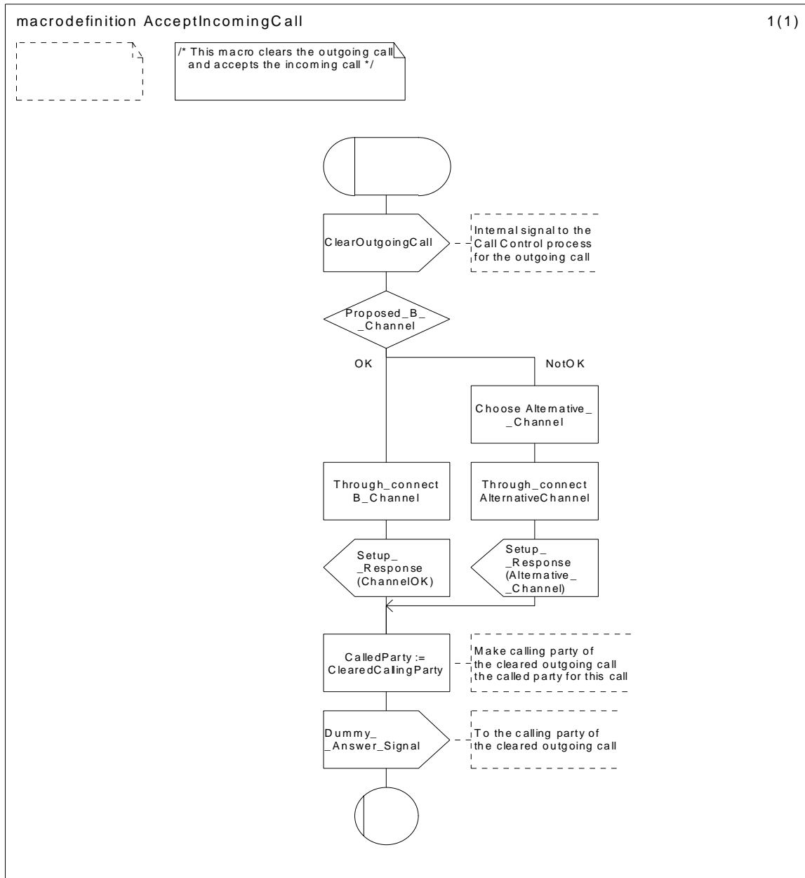
Figure C.3: SDL macro definition AcceptIncomingCall
