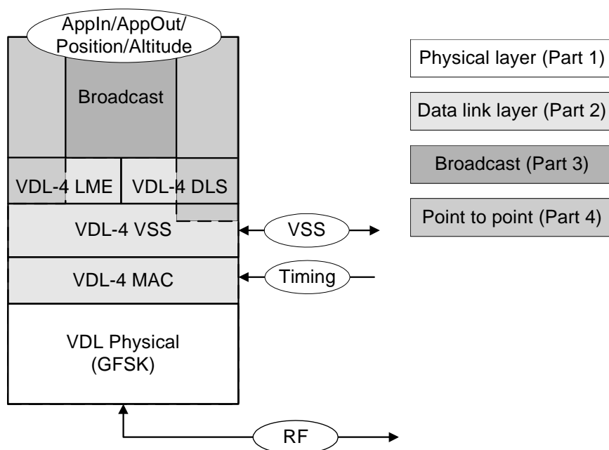
Figure 4.2: Structure of VDL Mode 4 ground station specifications
