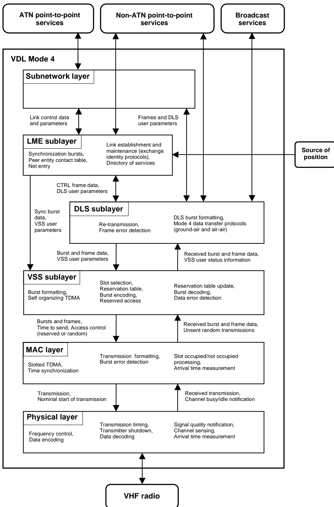
Figure 4.1: Layered structure of VDL Mode 4
