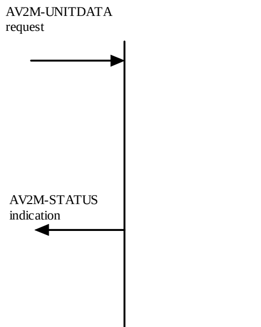
Figure 5.3: Sequence of primitives for an unsuccessful AV2MPDU transmission
