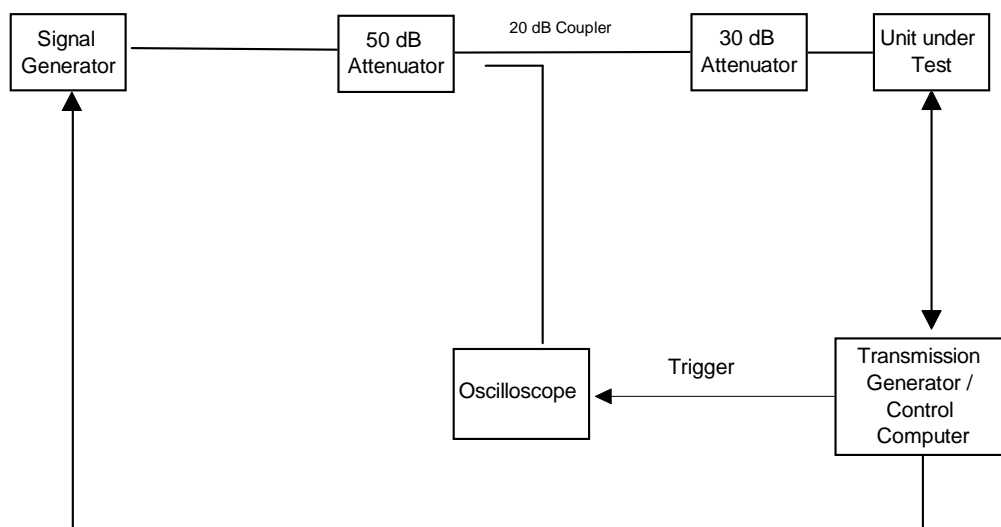
Figure 18: MAC Testbed
