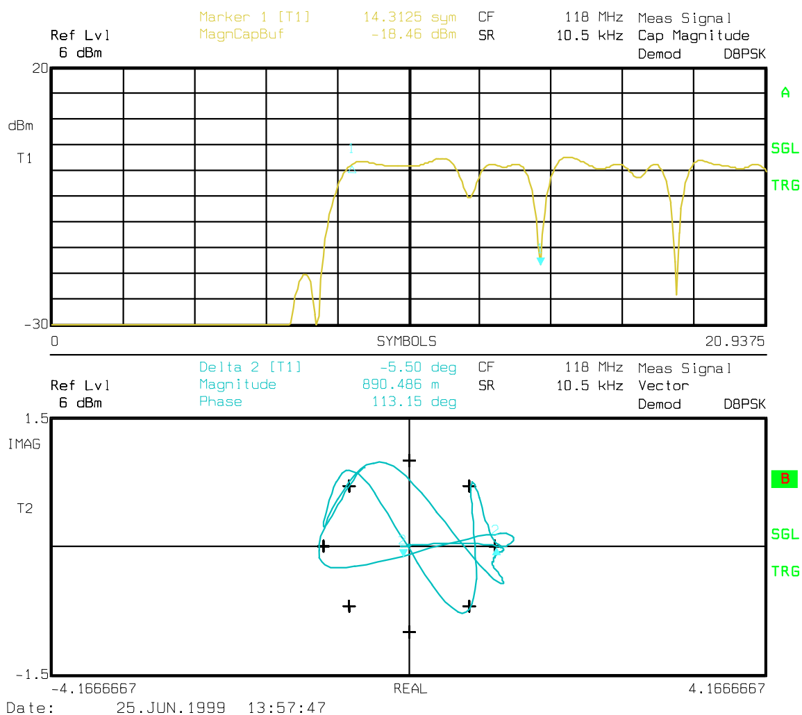
Figure 13: VSA displays constellation diagram illustrating rf rise-time
