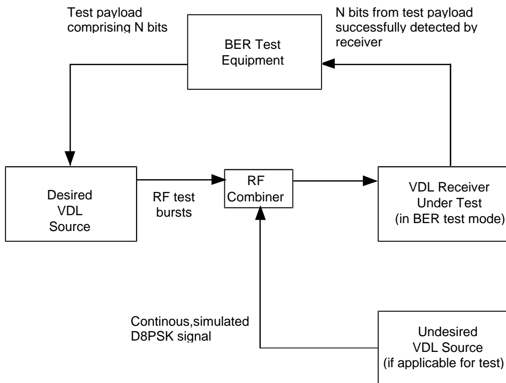
Figure 6: Receiver BER measurement
