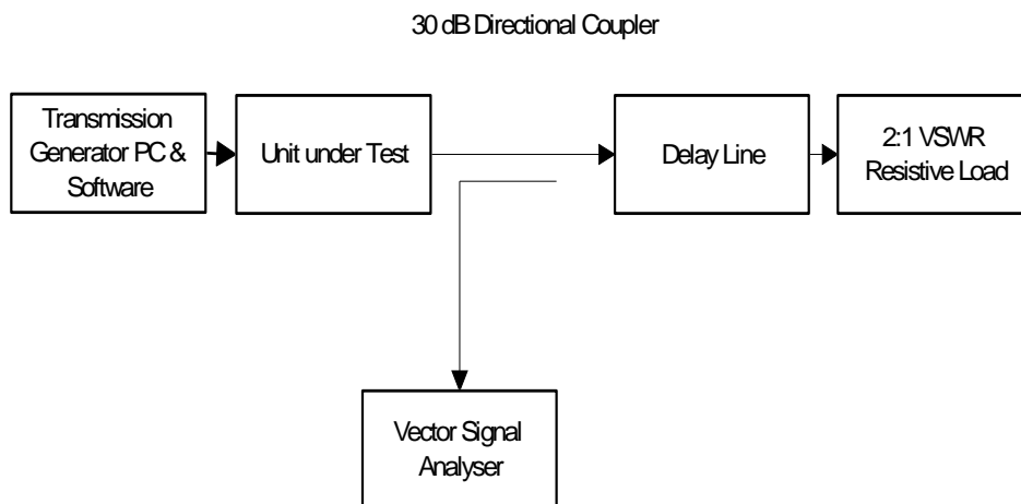
Figure 16: LOAD VSWR CAPABILITY
