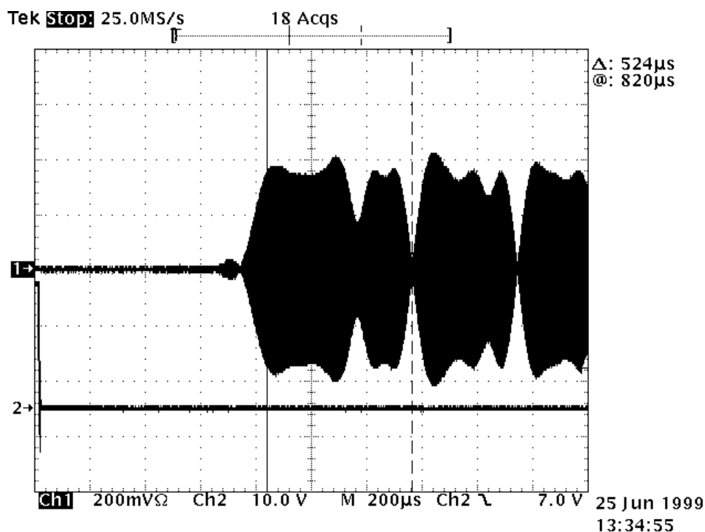
Figure 13a: Oscilloscope displays illustrating rf rise-time
