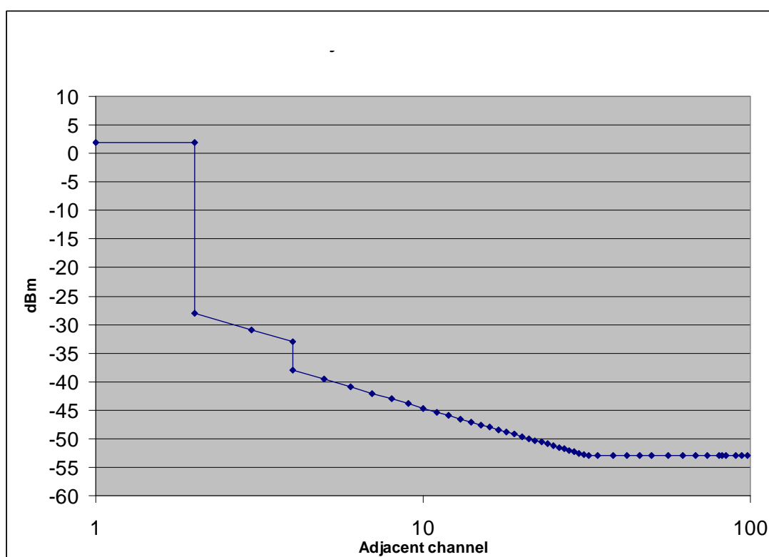
Figure 5: Maximum adjacent channel emissions
