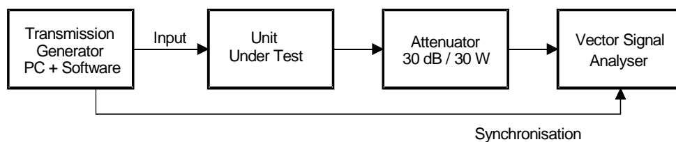
Figure 12: RF power rise and release time measurement also suitable for symbol constellation error
