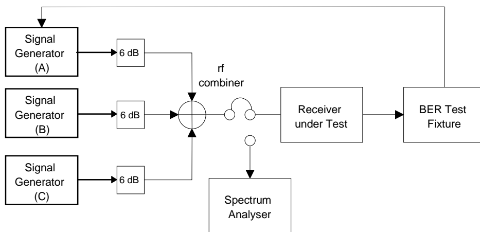
Figure 17: Intermodulation measurement
