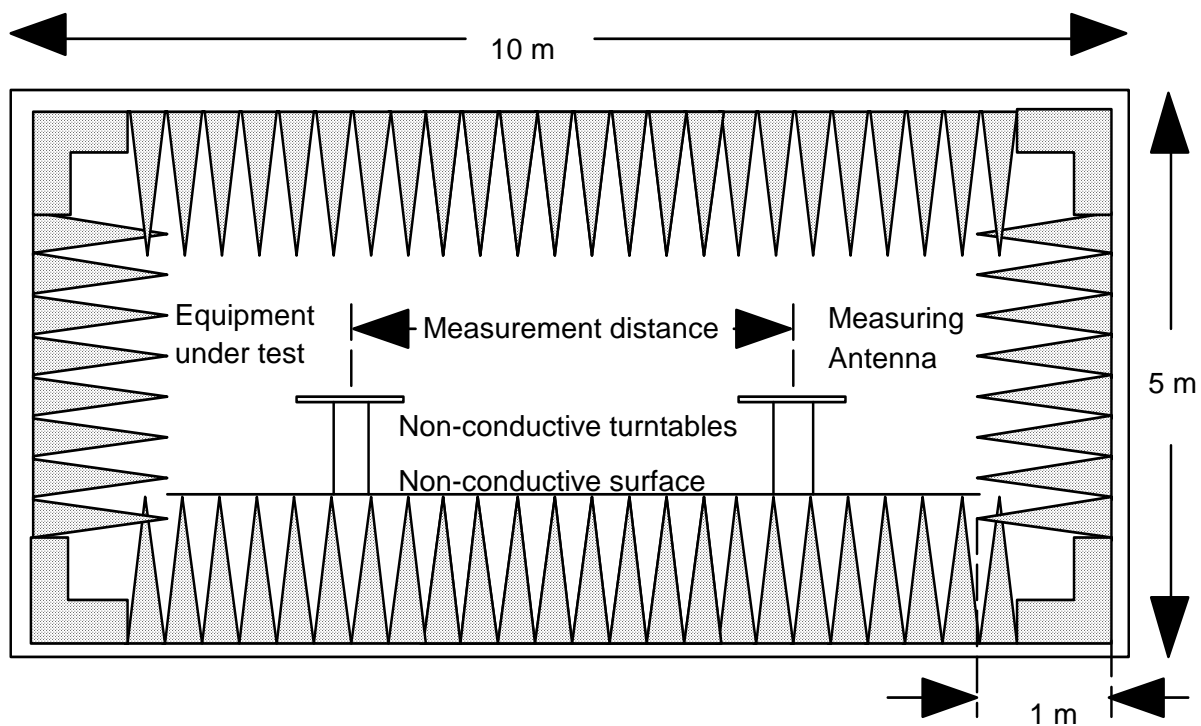
Ground plan
