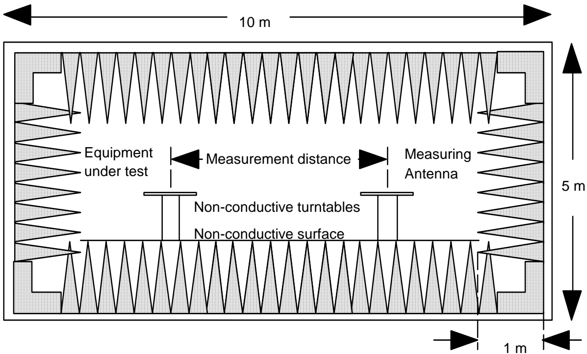
Ground plan
