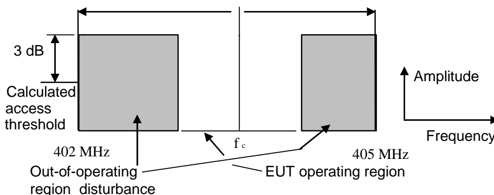
Figure 1: Spectrum Mask for Test of clause 10.1.1
