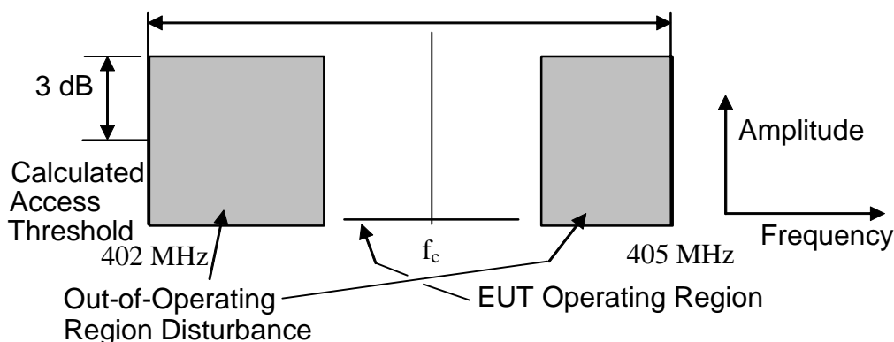
Figure 2: Spectrum Mask for Test of clause 10.2.1
