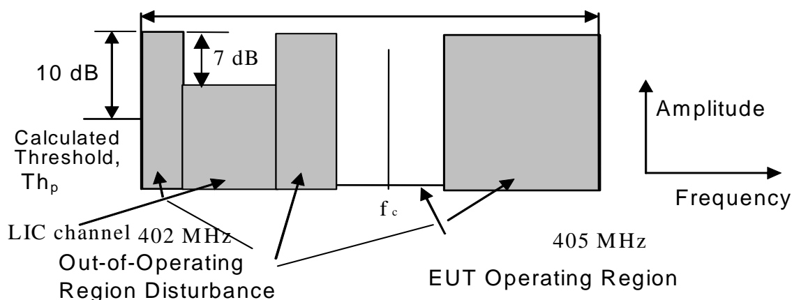
Figure 3: Spectrum Mask for Test of clause 10.4.1
