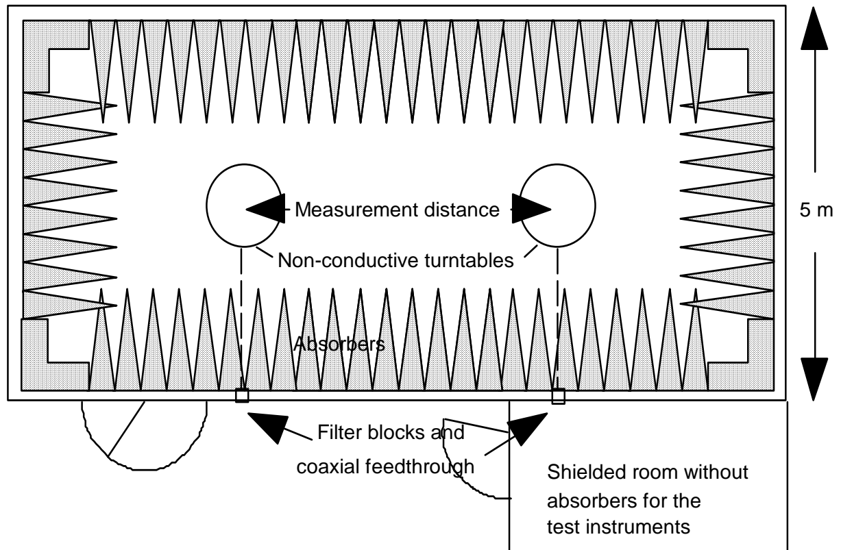
Ground plan
