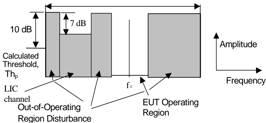
Figure 3: ULP-AMI Band
