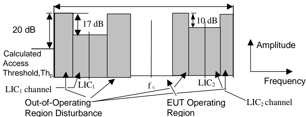
Figure 4: ULP-AMI Band
