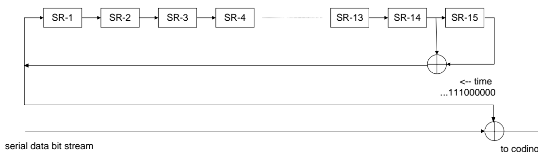
Figure 11: Randomizer
