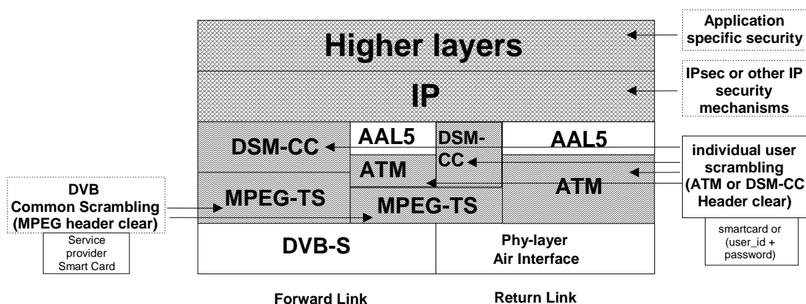
Figure 36: Security layers for satellite interactive network (example)
