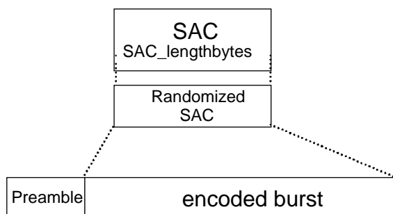
Figure 7: Composition of a SYNC burst
