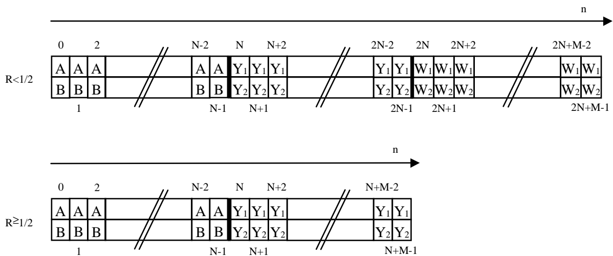
Figure 14: Encoded blocks (natural order)
