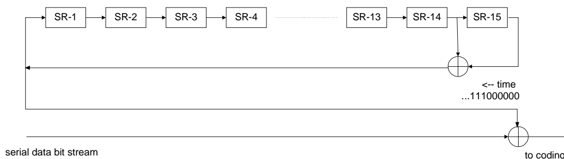
Figure 10: Randomizer
