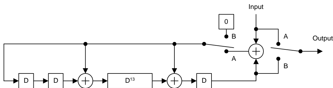
Figure 11: CRC calculation
