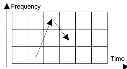
Figure 20: Fixed-slot MF-TDMA
