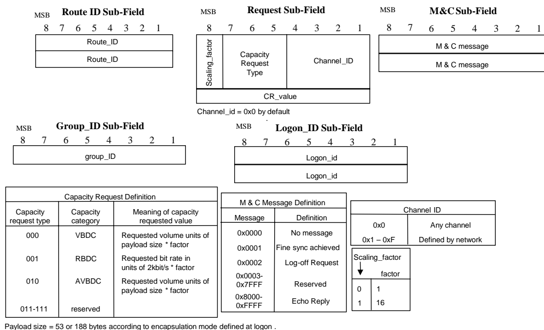
Figure 17: Composition of the SAC field
