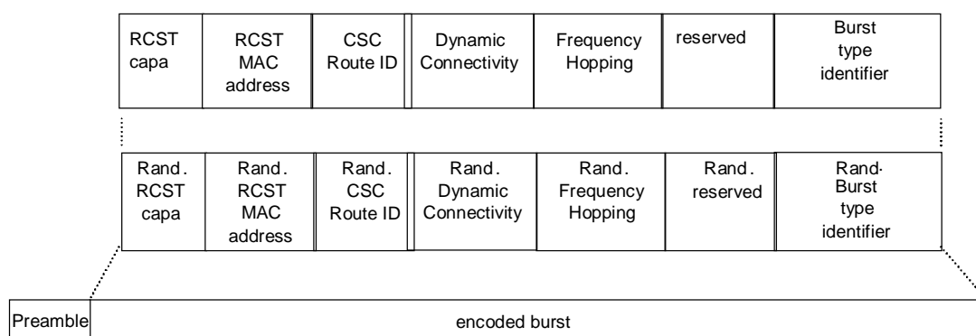
Figure 9: Composition of a CSC burst
