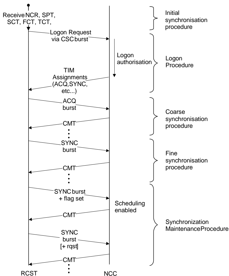
Figure 26: Example of RCST network entry signalling flow
