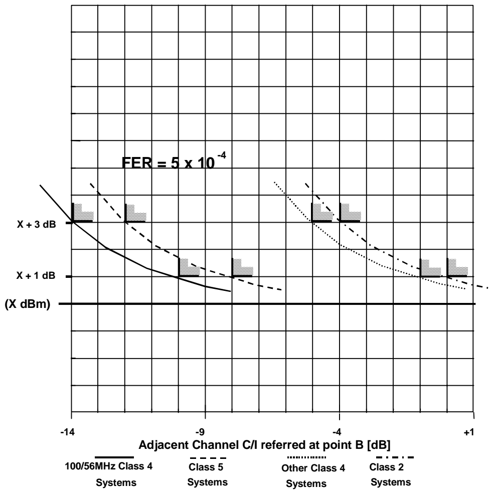
Receiver Input Level at Reference Point C relative to FER = 5 x 10 -4 threshold
