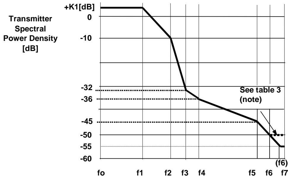
Figure 2b: Limits of spectral power density for Class 5 systems
