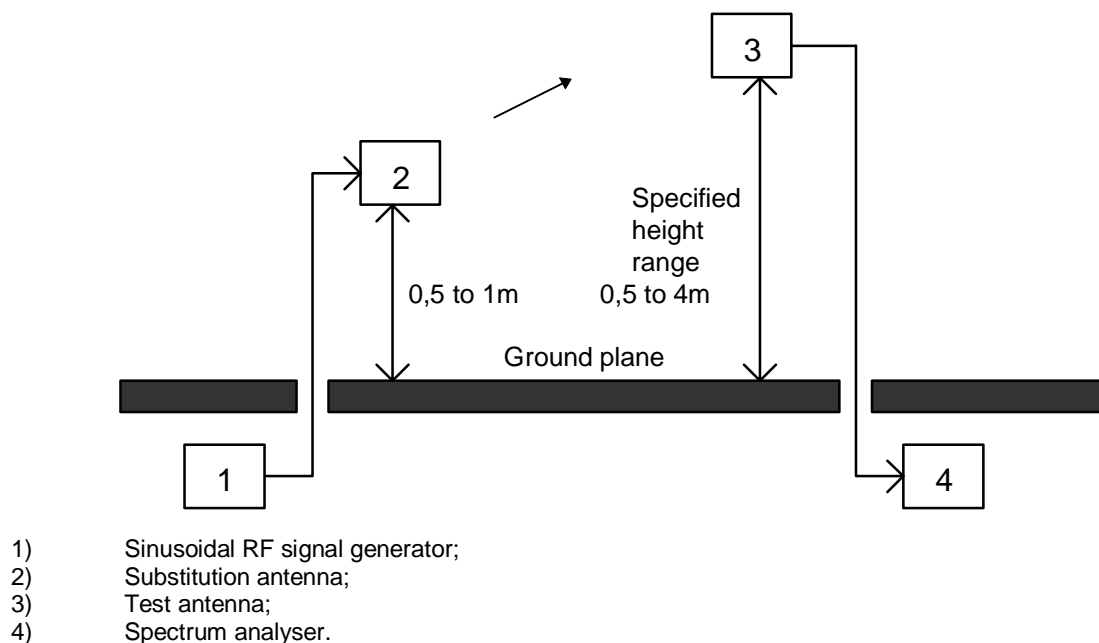
Figure 4: Measurement arrangement No.2
