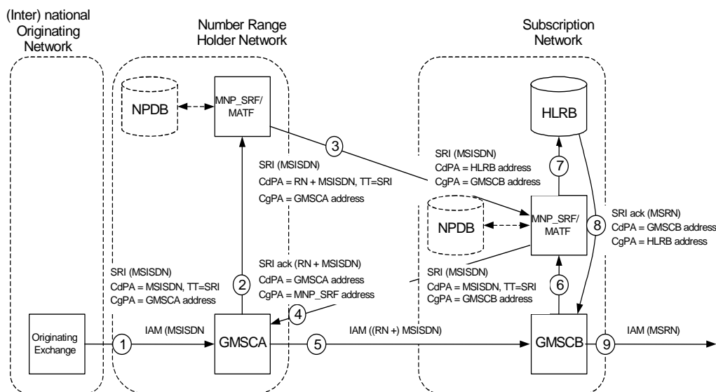
Figure C.3.5: National or international originated call to a ported number where indirect routeing with reference to the subscription network is used
