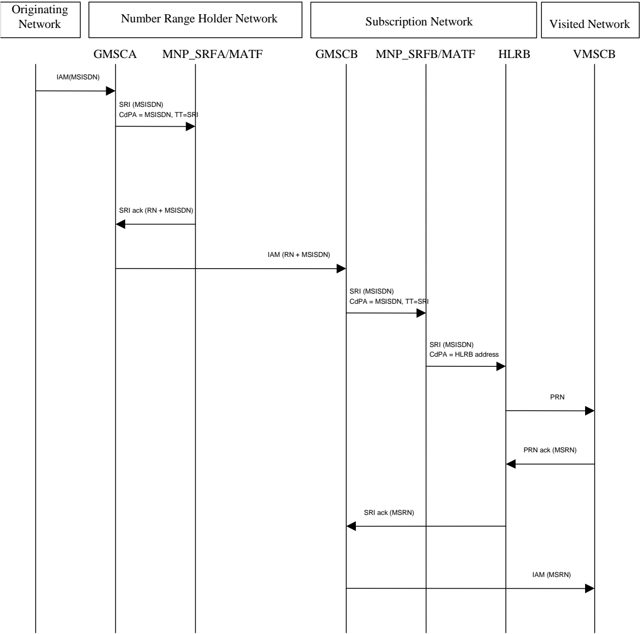
Figure C.4.5: Successful delivery of a call to a ported number via indirect routeing
