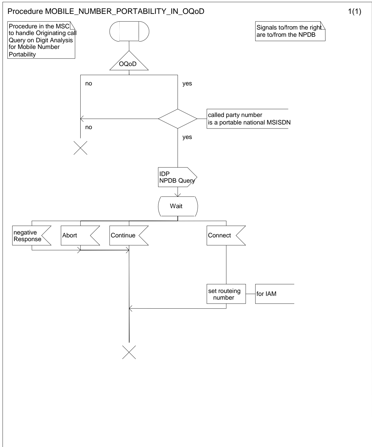
Figure A.3.3: Procedure MOBILE_NUMBER_PORTABILITY_IN_OQoD
