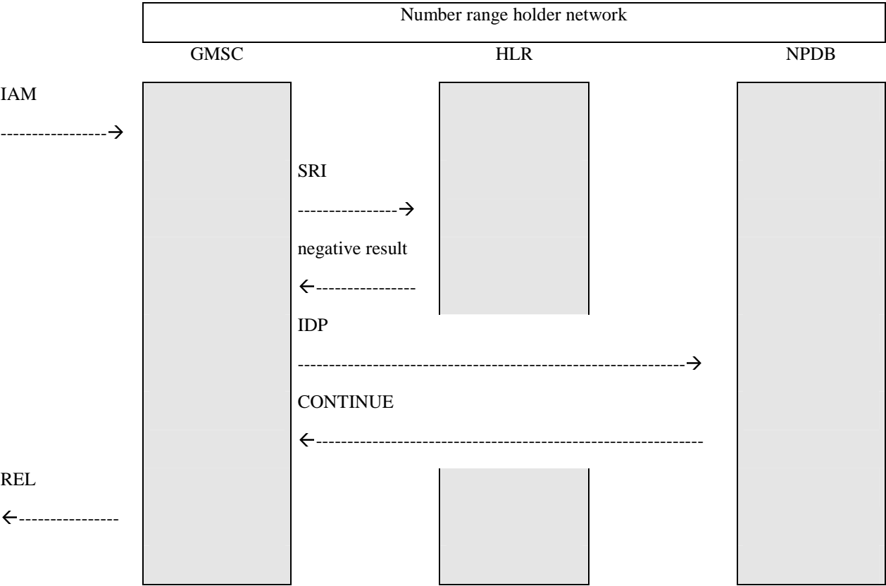
Figure A.2.2: Information flow for unsuccessful QoHR (misdialled unallocated number)
