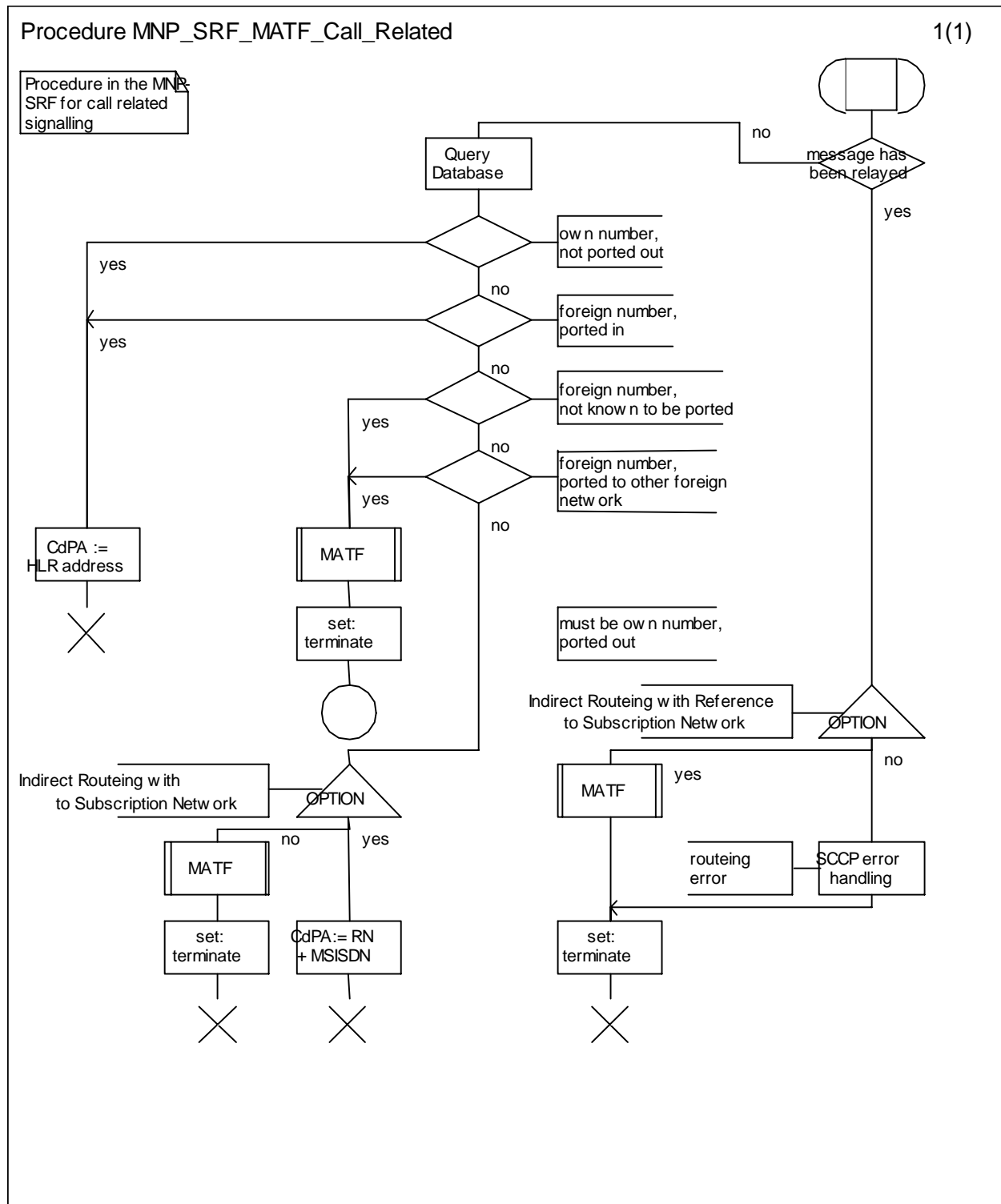
Figure C.2.1.1: Procedure MNP_SRF_MATF_Call_Related
