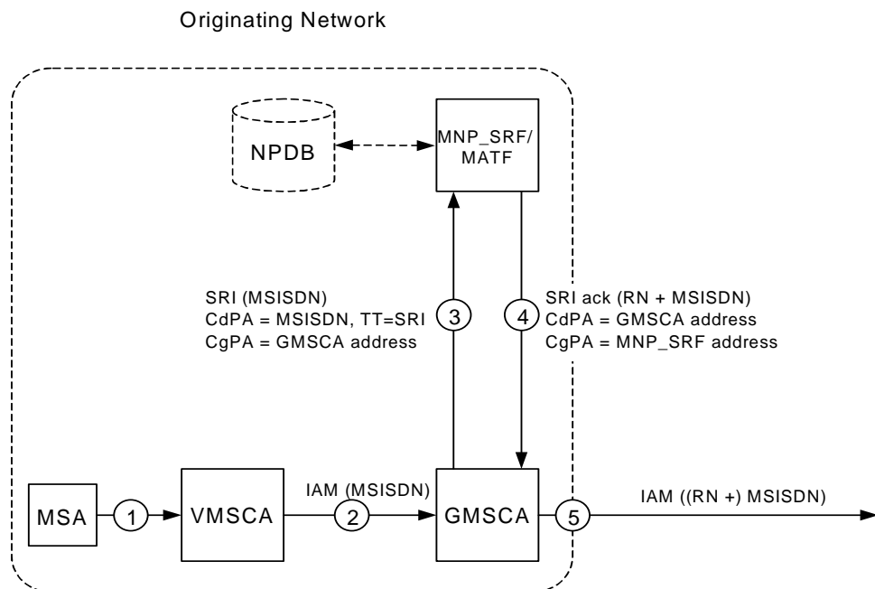
Figure C.3.3: National mobile originated call to a ported number via direct routeing
