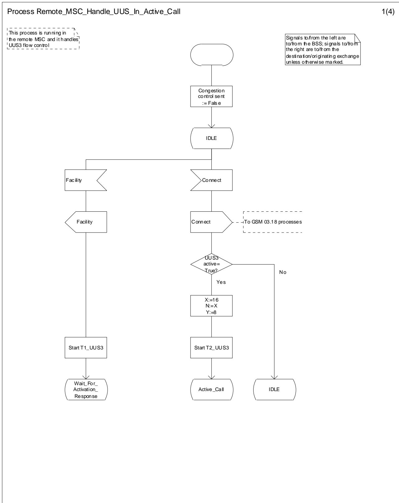
Figure 9.4.3.1: Process Remote_MSC_Handle_UUS_In_Active_Call (sheet 1)
