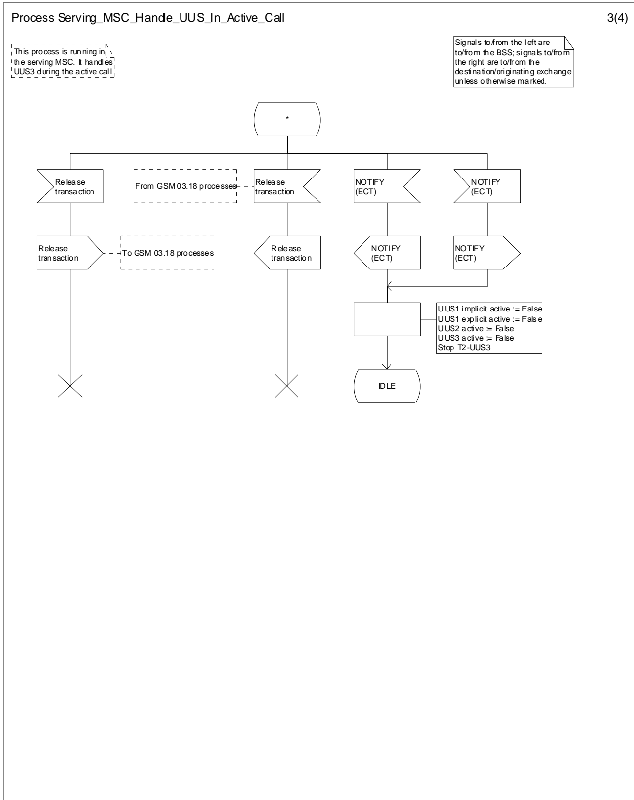
Figure 9.4.1.1: Process Serving_MSC_Handle_UUS_In_Active_Call (sheet 3)
