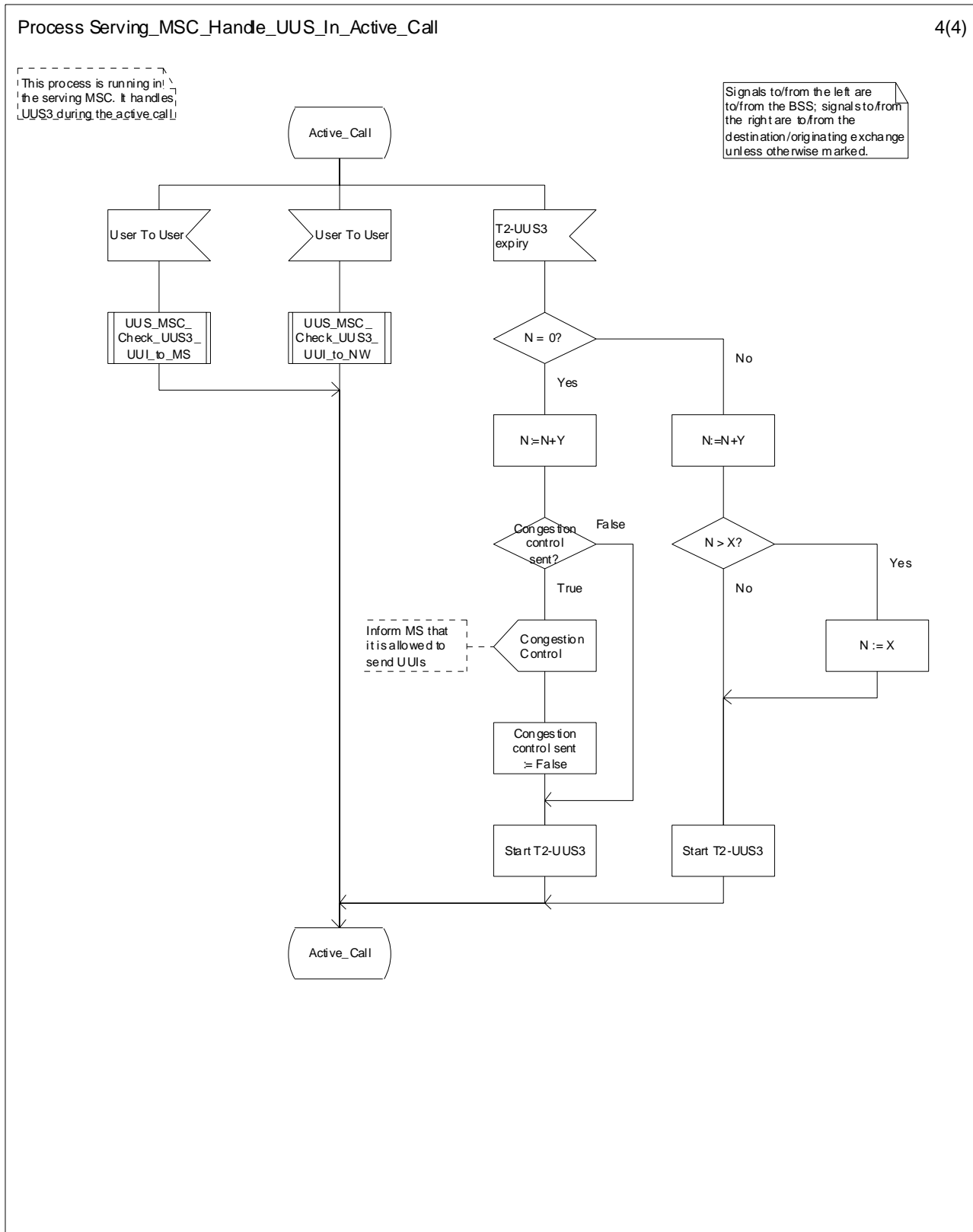
Figure 9.4.1.1: Process Serving_MSC_Handle_UUS_In_Active_Call (sheet 4)
