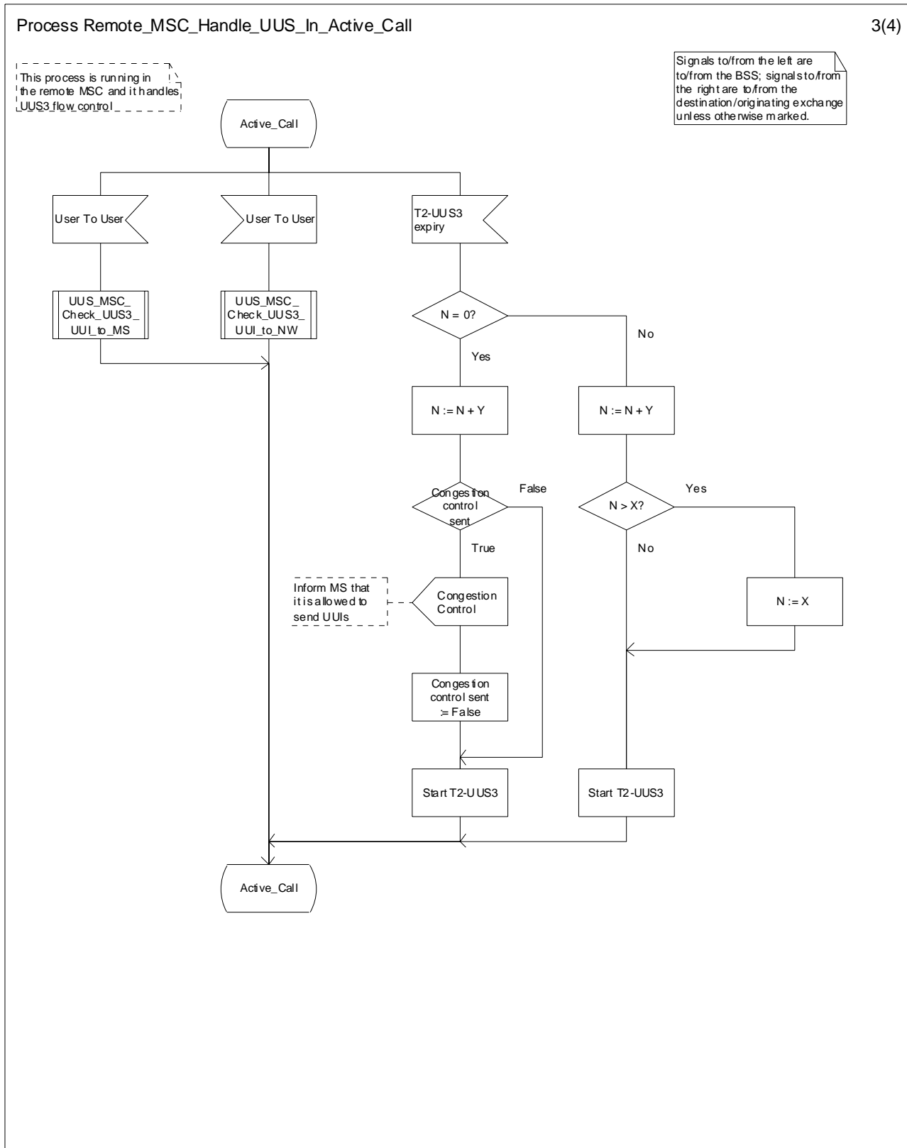
Figure 9.4.3.1: Process Remote_MSC_Handle_UUS_In_Active_Call (sheet 3)
