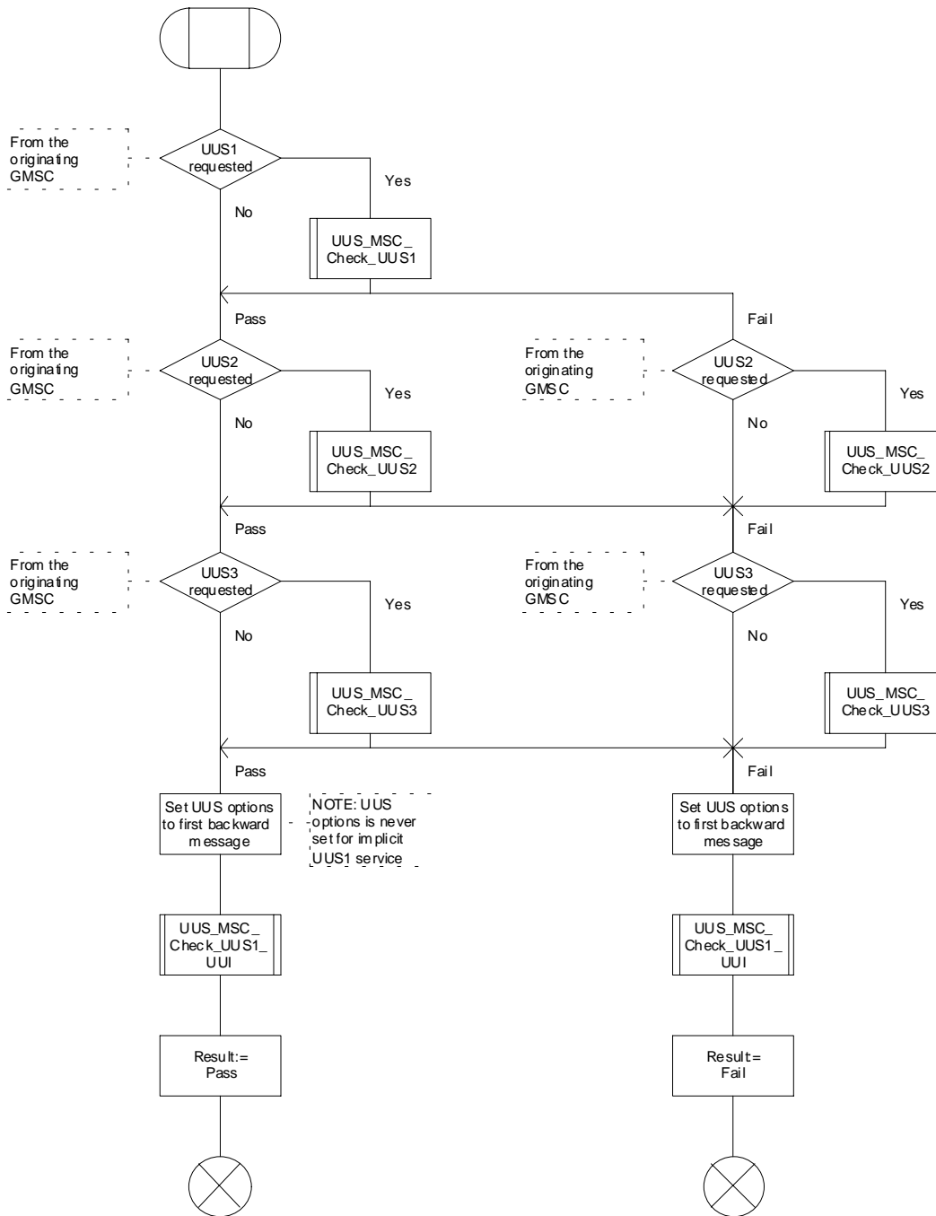
Figure 9.2.2.1: Procedure UUS_ICH_Check_Support
