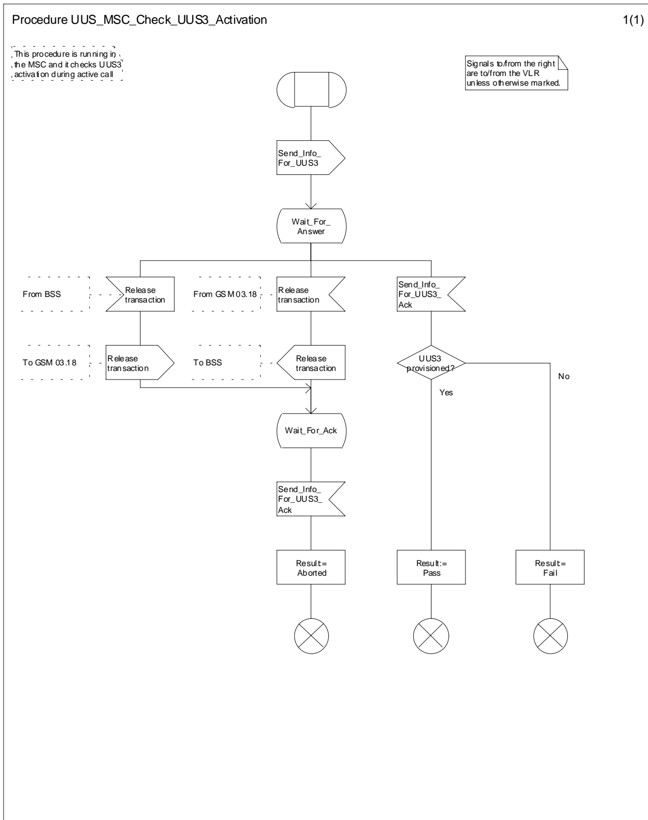
Figure 9.4.1.2: Procedure UUS_MSC_Check_UUS3_Activation
