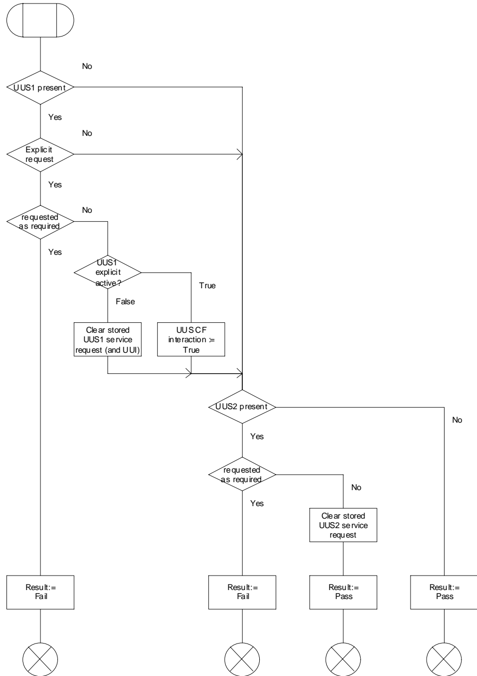
Figure 9.2.2.2: Procedure UUS_ICH_Check_Forwarding
