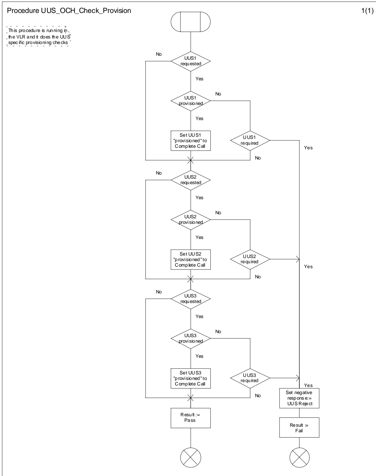
Figure 9.1.2.1: Procedure UUS_OCH_Check_Provision
