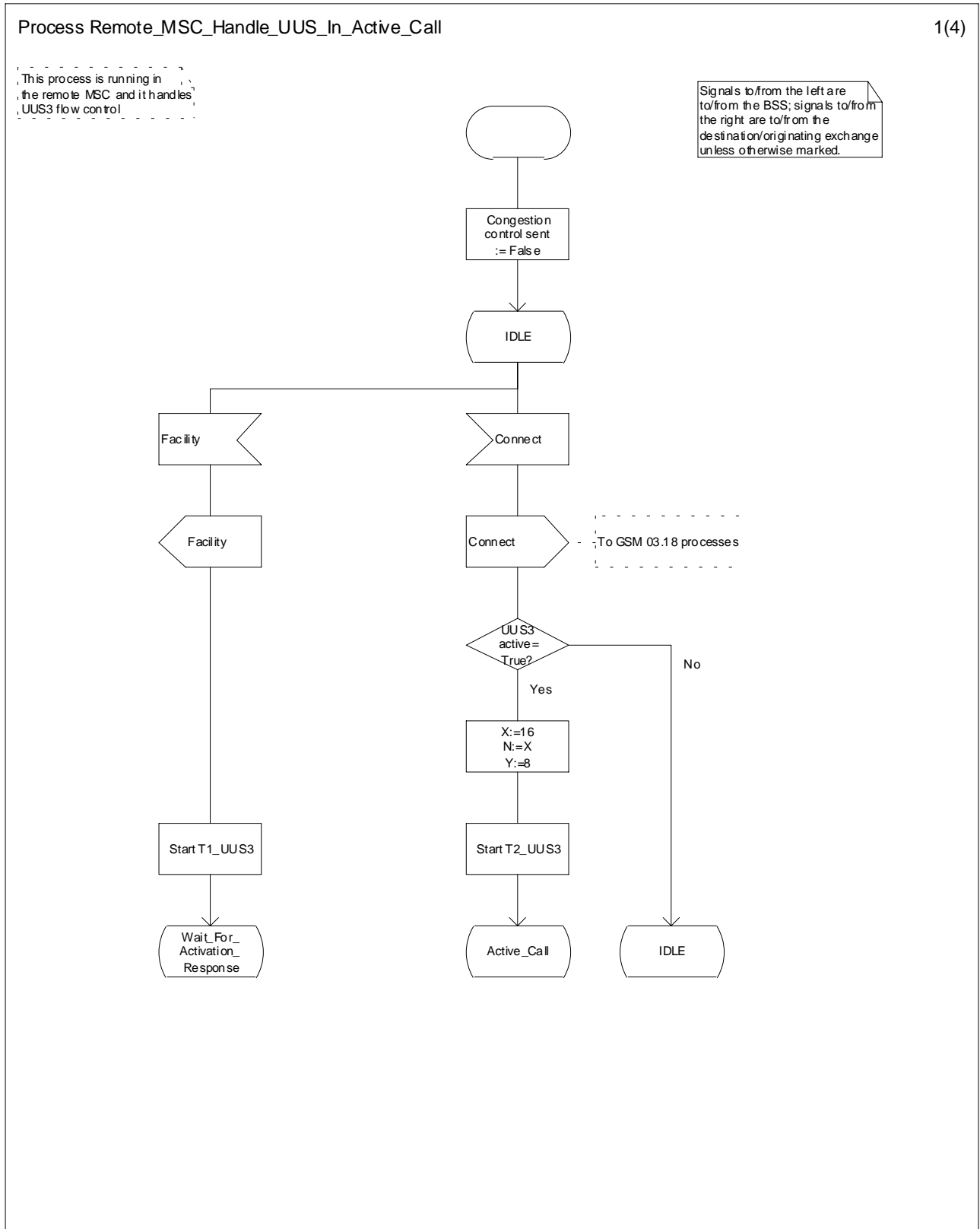
Figure 9.4.3.1: Process Remote_MSC_Handle_UUS_In_Active_Call (sheet 1)
