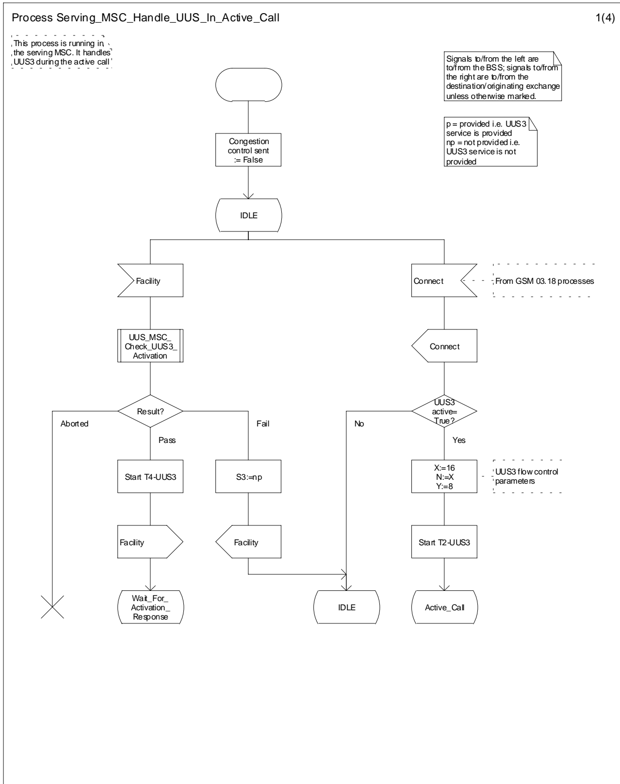
Figure 9.4.1.1: Process Serving_MSC_Handle_UUS_In_Active_Call (sheet 1)
