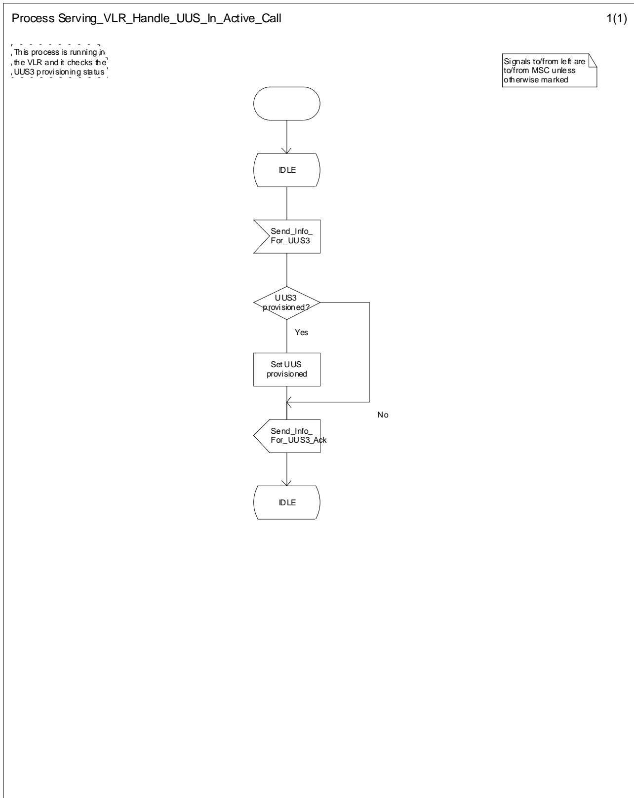
Figure 9.4.2.1: Process Serving_VLR_Handle_UUS_In_Active_Call
