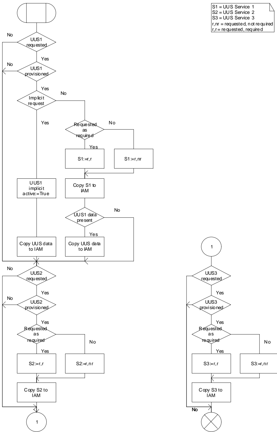
Figure 9.1.1.2: Procedure UUS_OCH_Set_Info_In_IAM
