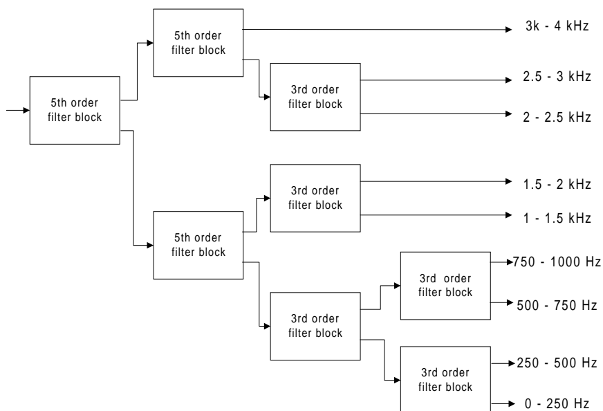
Figure 3.2: Filter bank
