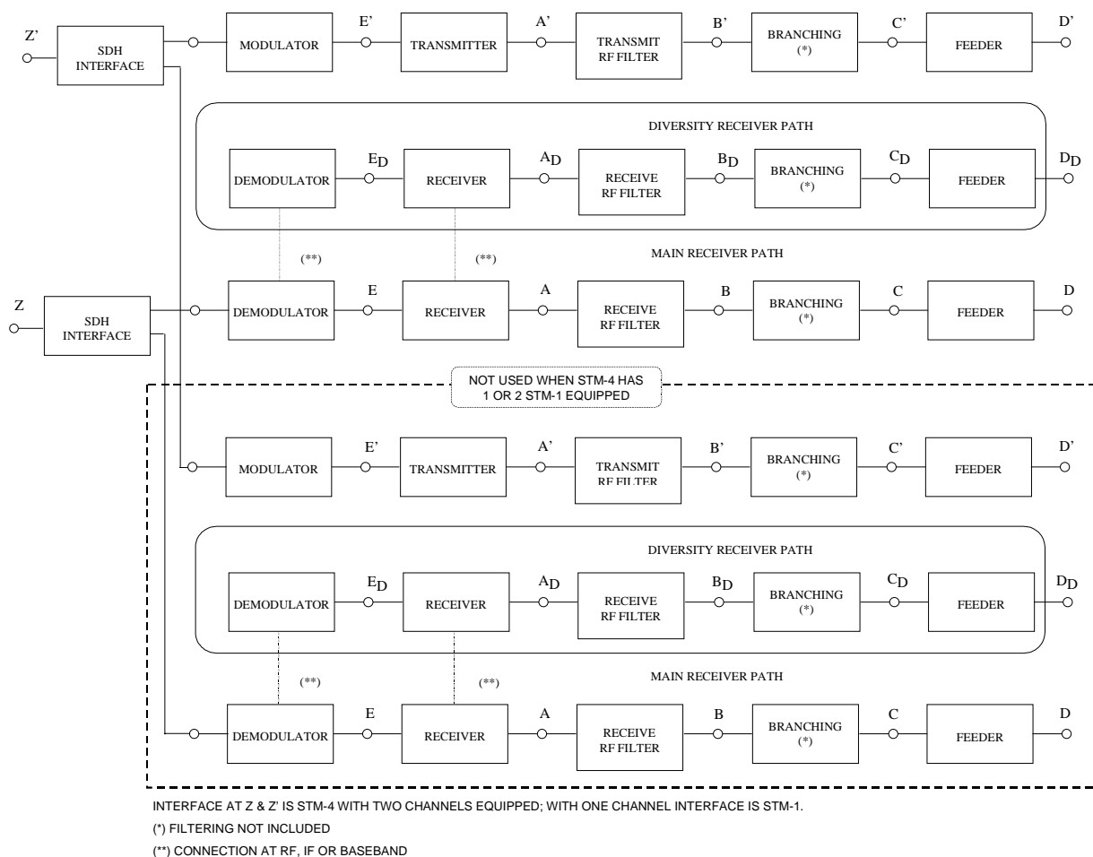
Figure 1: Block diagram
