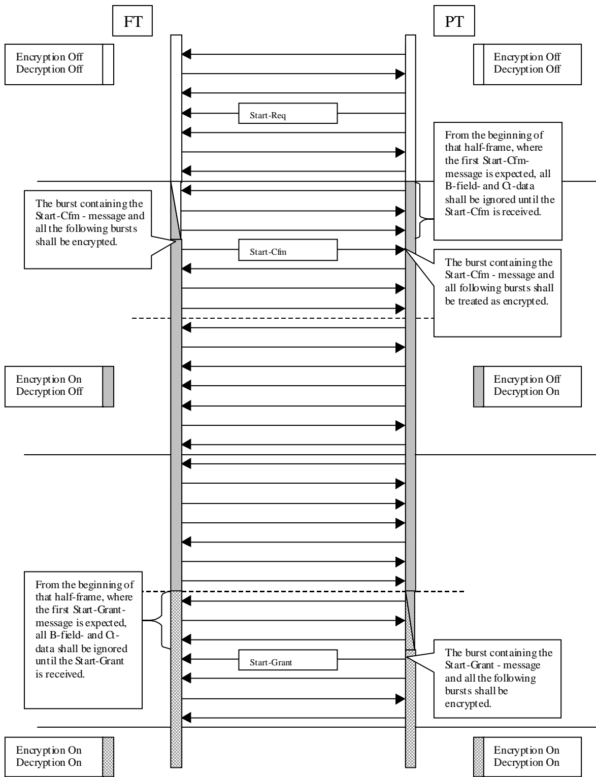
Figure 17: Encryption procedures
