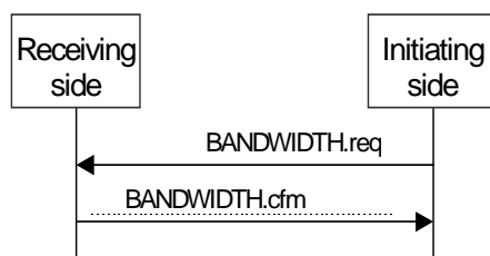
Figure 7: Bandwidth negotiation
