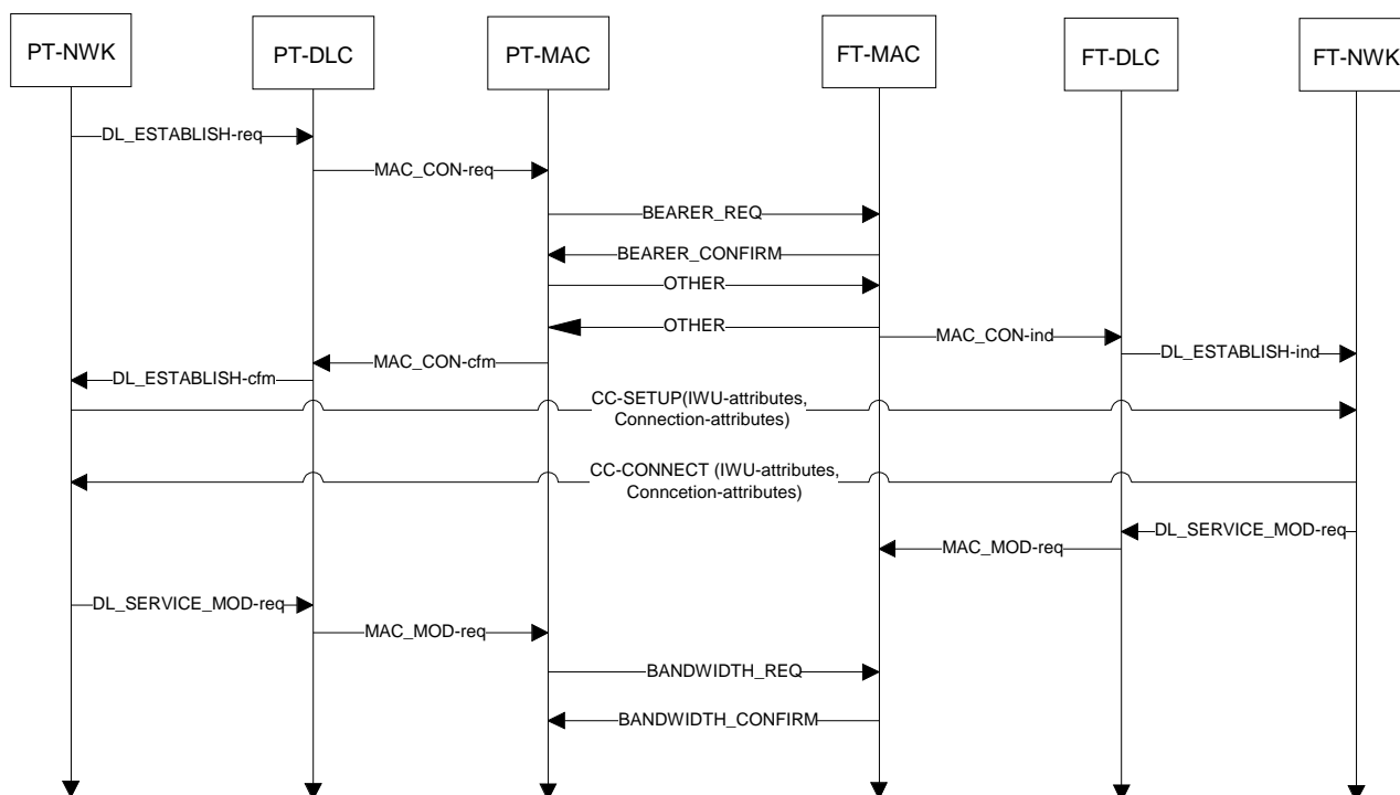
Figure 12: Service/parameters negotiation interlayer exchange
