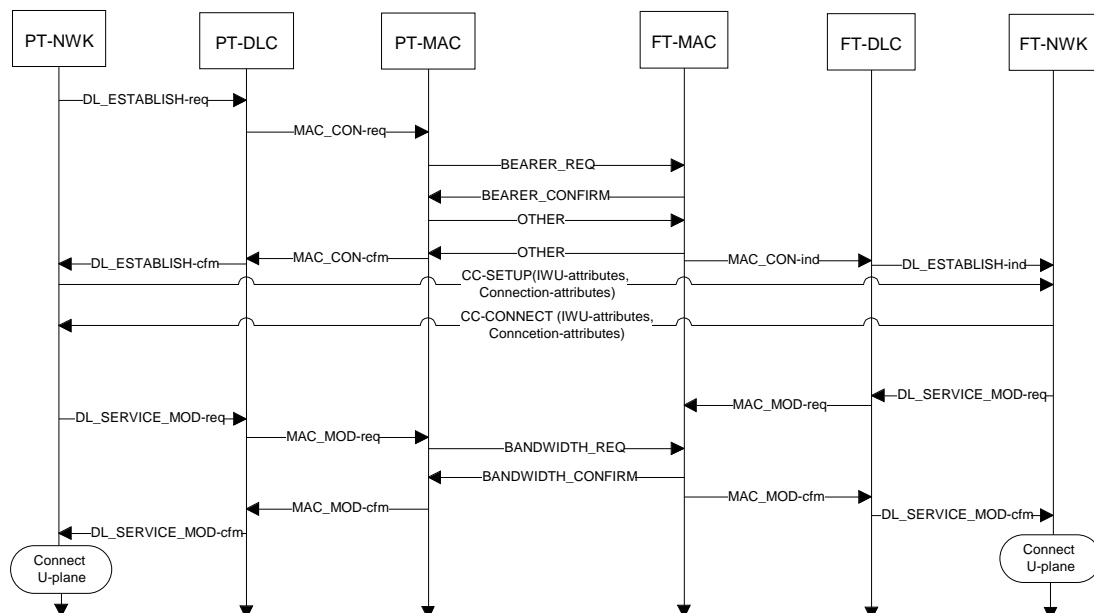
Figure 18: Example of connection of the U-plane in case of Service negotiation
