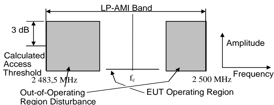
Figure 2: Spectrum Mask for Test of clauses 10.2.1 and 10.2.2
