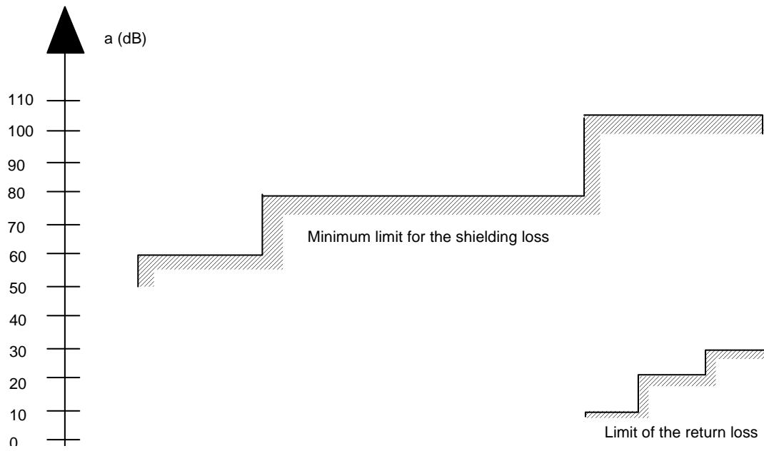
Figure A.5: Specification for shielding and reflections
