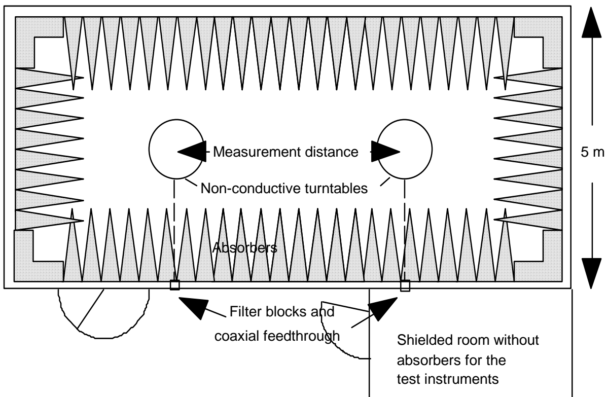
Ground plan
