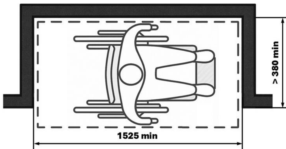
Figure 8.10: Manoeuvring Clearance in an a space bounded on 3 sides, Parallel Approach
