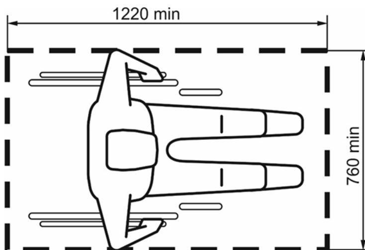
Figure 8.8: Clear floor area in front of the ICT
