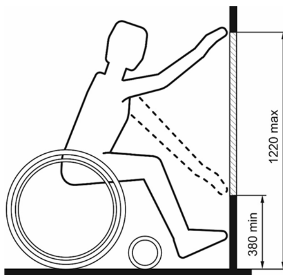
Figure 8.1: Unobstructed forward reach
