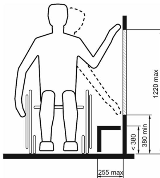
Figure 8.4: Unobstructed side reach
