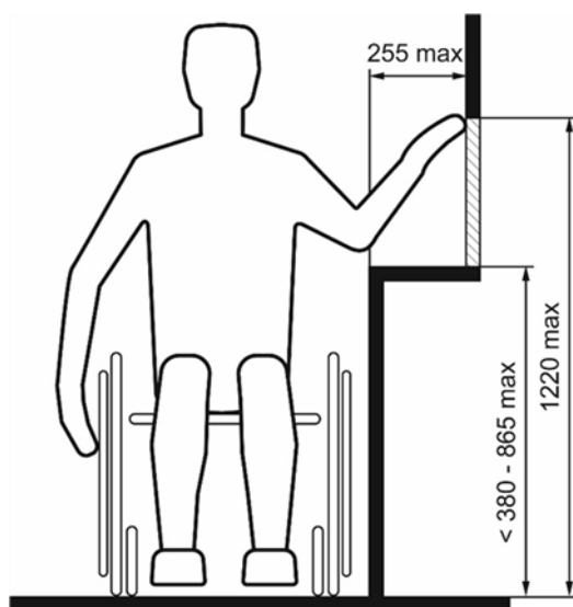
Figure 8.5a: Obstructed side reach \leq 255 mm
