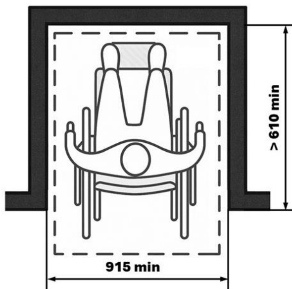
Figure 8.9: Manoeuvring Clearance in a space bounded on 3 sides, Forward Approach
