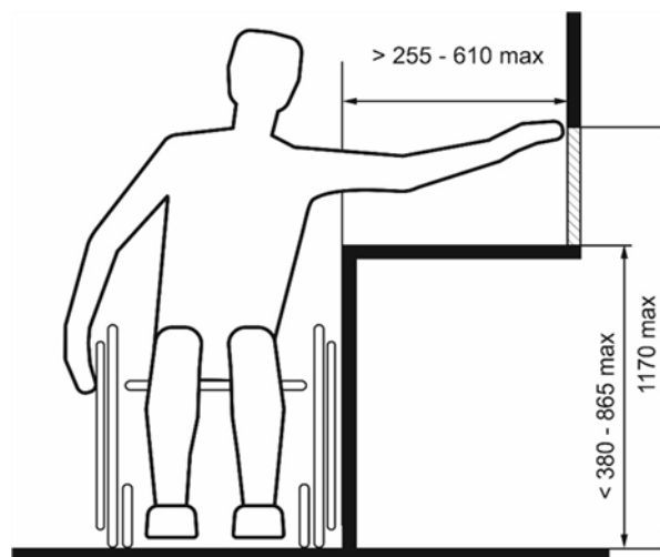
Figure 8.5b: Obstructed side reach > 255 mm
