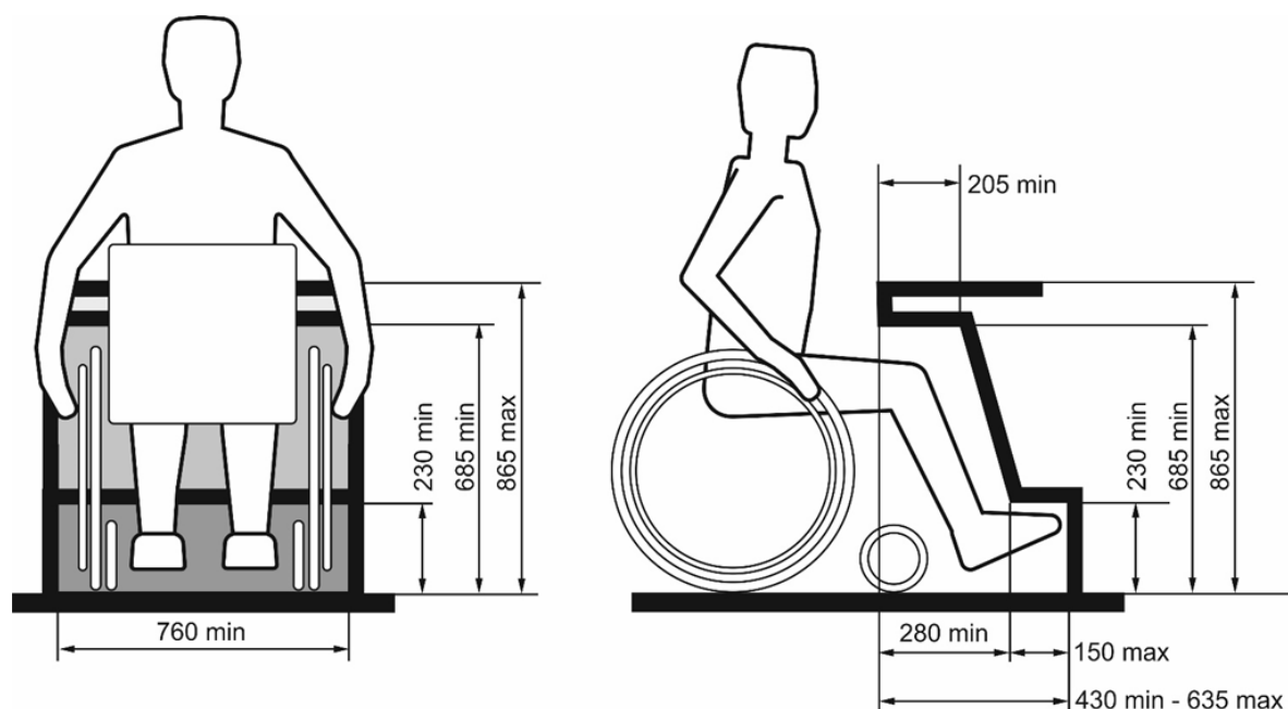
Figure 8.2: Knee and toe clearance underneath an obstruction
