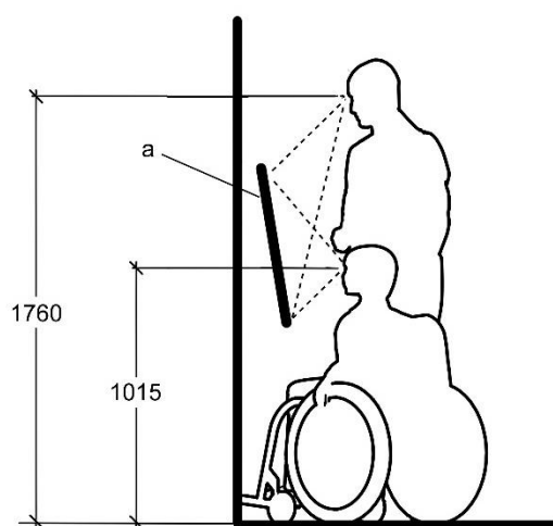
Figure 8.11: Information legible when standing and sitting
