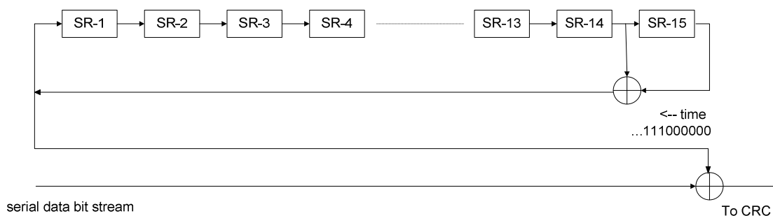
Figure 7-9: PRBS Randomizer
