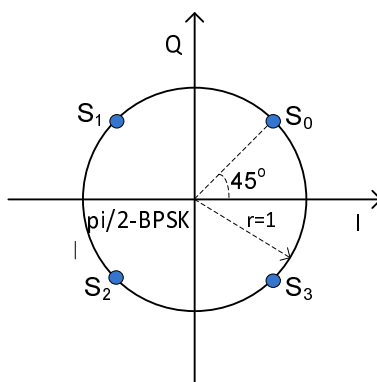
Figure 7-19: pi/2-BPSK constellation
