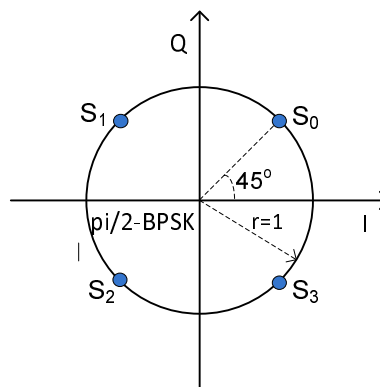
Figure 7-19: pi/2-BPSK constellation
