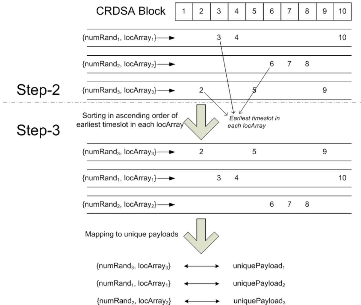
Figure 7-6: Example locArray sorting with \text{nofSlots}=10 , \text{nofInstances}=3 and 3 unique payloads
