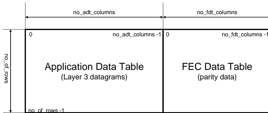
Figure 5-1: LL-FEC frame
