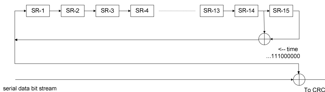
Figure 7-9: PRBS Randomiser
