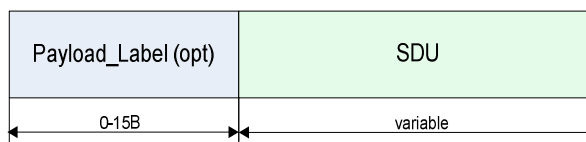
Figure 7-4: Frame PDU Format for a Frame Dedicated to Internal Signalling (Logon and Control)
