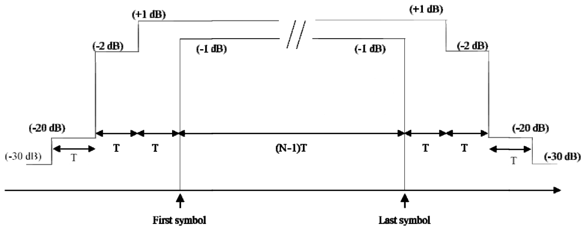
Figure 7-22: Burst power envelope mask for CC-CPM bursts
