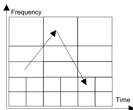
Figure 7-28: Dynamic MF-TDMA
