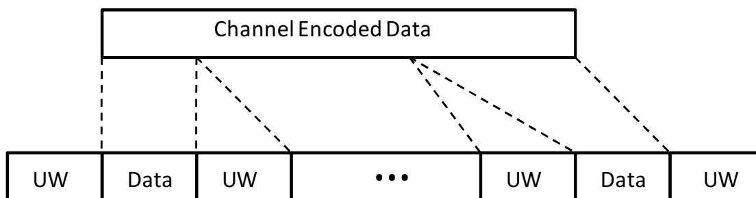
Figure 7-17: CC-CPM burst structure
