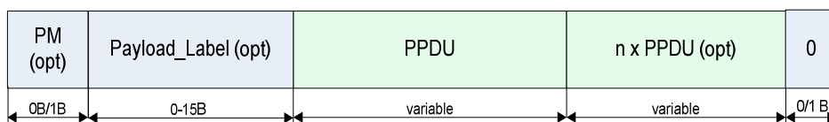
Figure 7-3: Frame PDU Format for a Frame Supporting User Traffic
