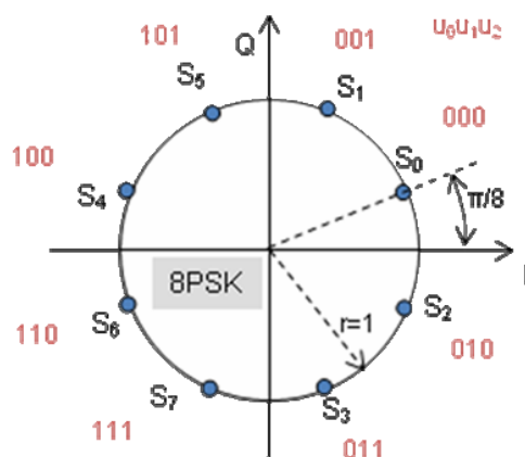
Figure 7-19: 8-PSK constellation
