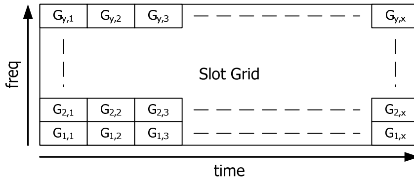
Figure 7-25: A Frame Implemented by 'x' BTUs of Type 'G' per Carrier in 'y' Adjacent Carriers
