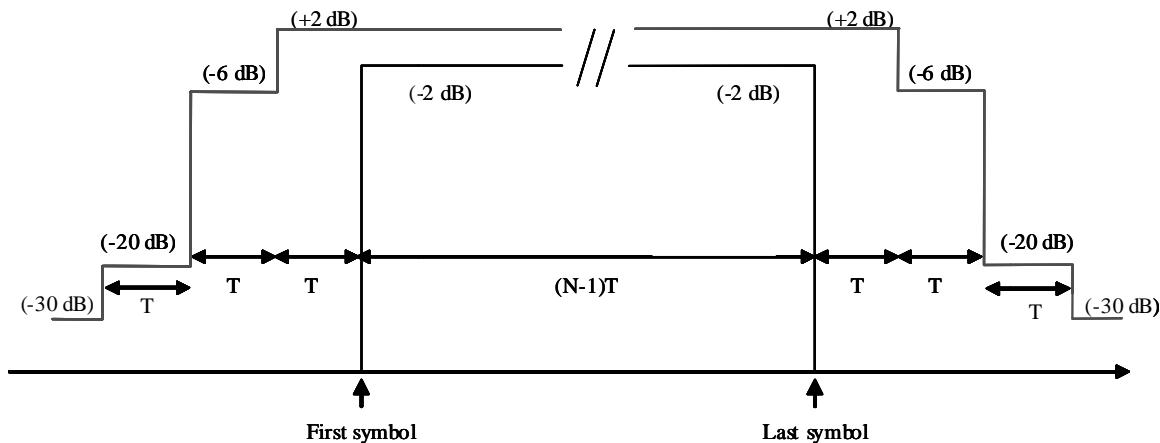
Figure 7-21: Burst power envelope mask for TC-LM bursts
