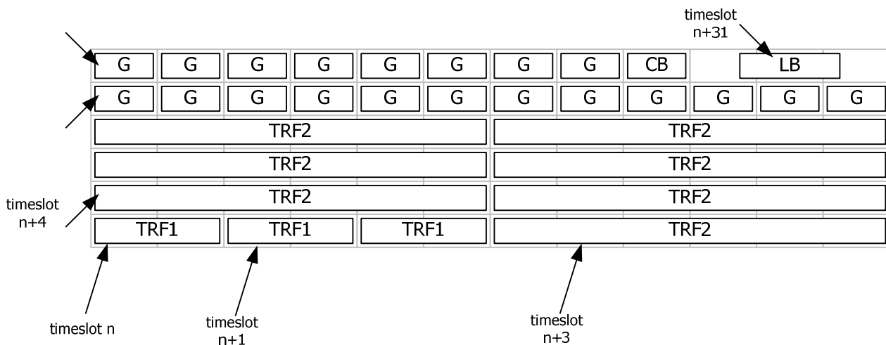
Figure 7-26: Example of the Composition of a Frame Type
