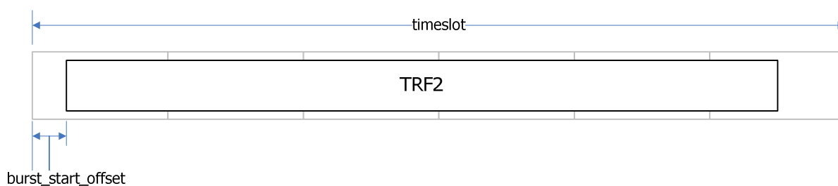
Figure 7-27: Example of a Burst in a Timeslot Built from 6 BTUs
