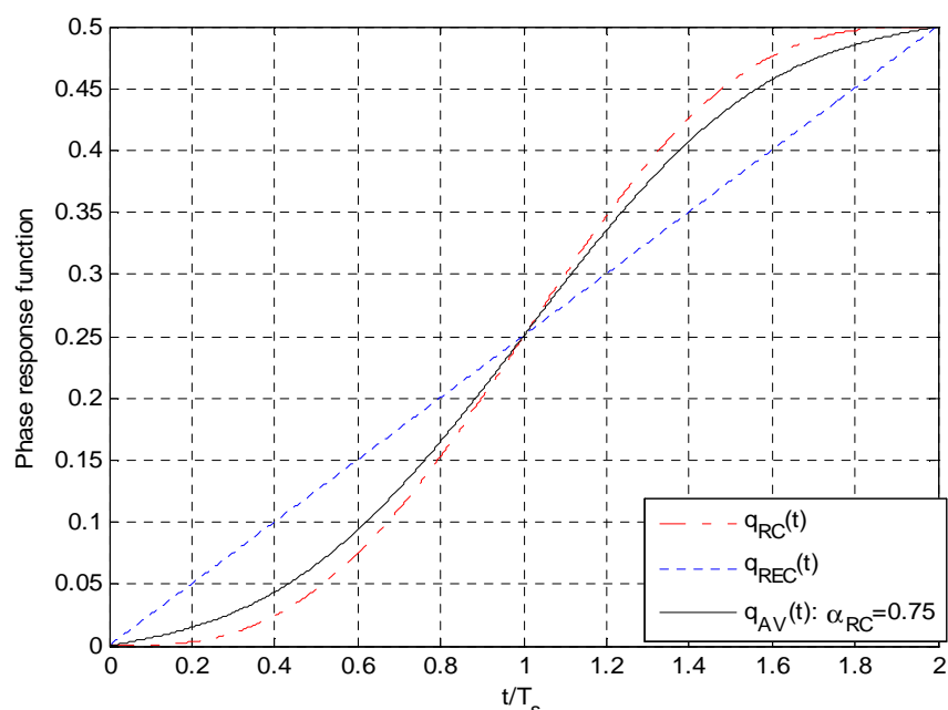
Figure 7-20: Phase response for RC, REC and AV pulse shapes
