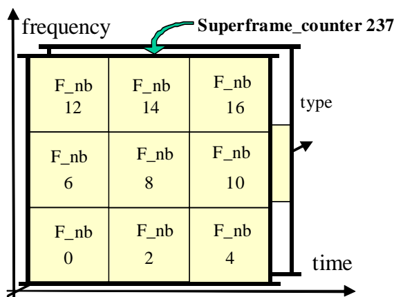
Figure 7-23: Example of superframe composition
