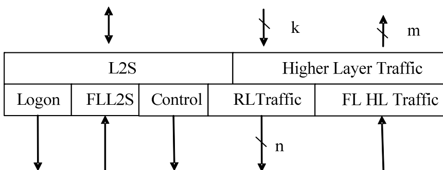
Figure 4-2: Segmentation of the Lower Layers at an RCST
