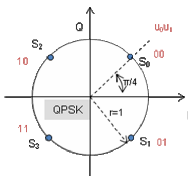
Figure 7-18: QPSK constellation
