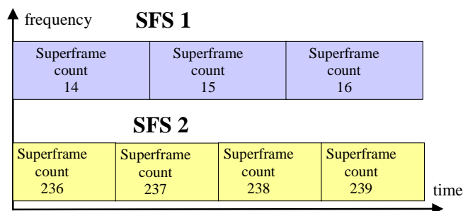
Figure 7-24: Example of superframe sequences
