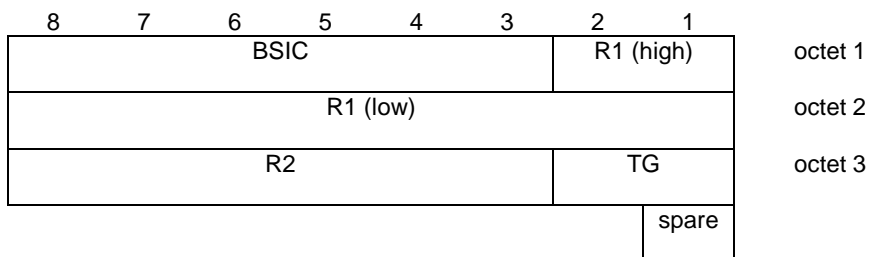
Figure 9.3b/GSM 04.18: COMPACT Frame synchronization information element
