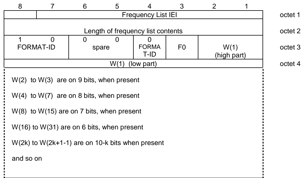
Figure 10.5.36/GSM 04.18 Frequency List information element (Range 1024 format)
