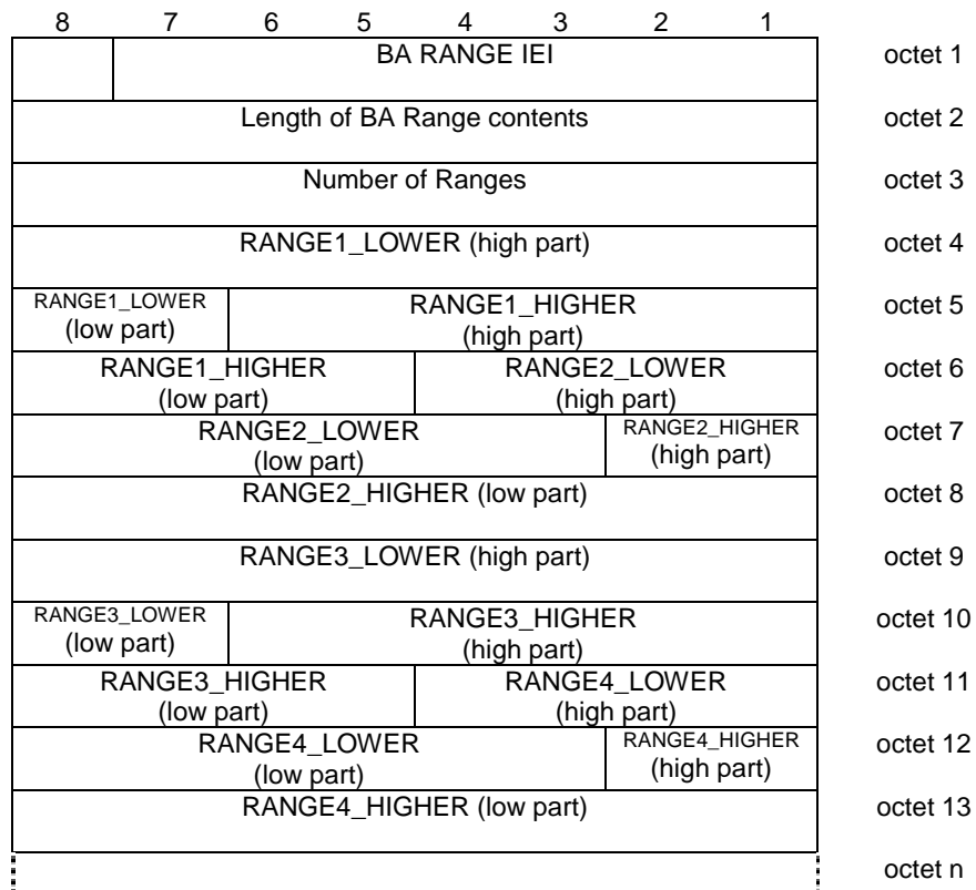
Figure 10.5.12/GSM 04.18 BA RANGE information element
