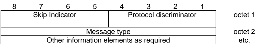
Figure 10.1/GSM 04.18 General message organization example
