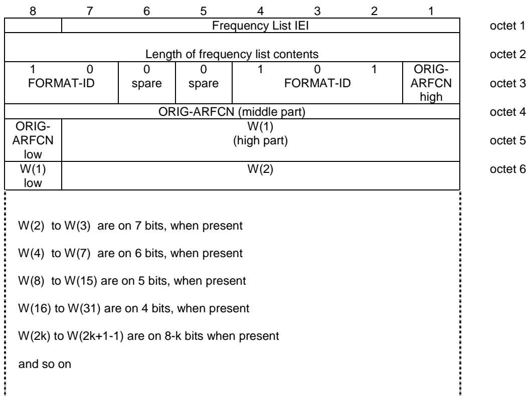
Figure 10.5.38/GSM 04.18 Frequency List information element (Range 256 format)
