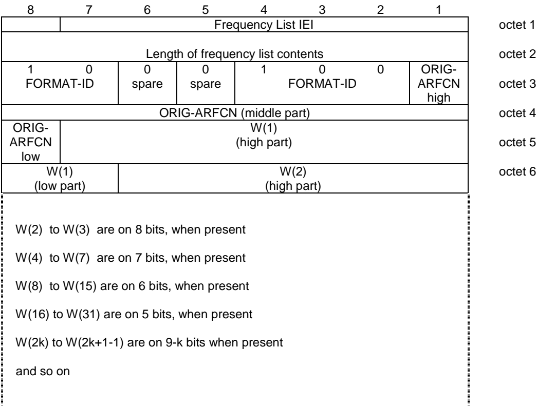
Figure 10.5.37/GSM 04.18 Frequency List information element (Range 512 format)
