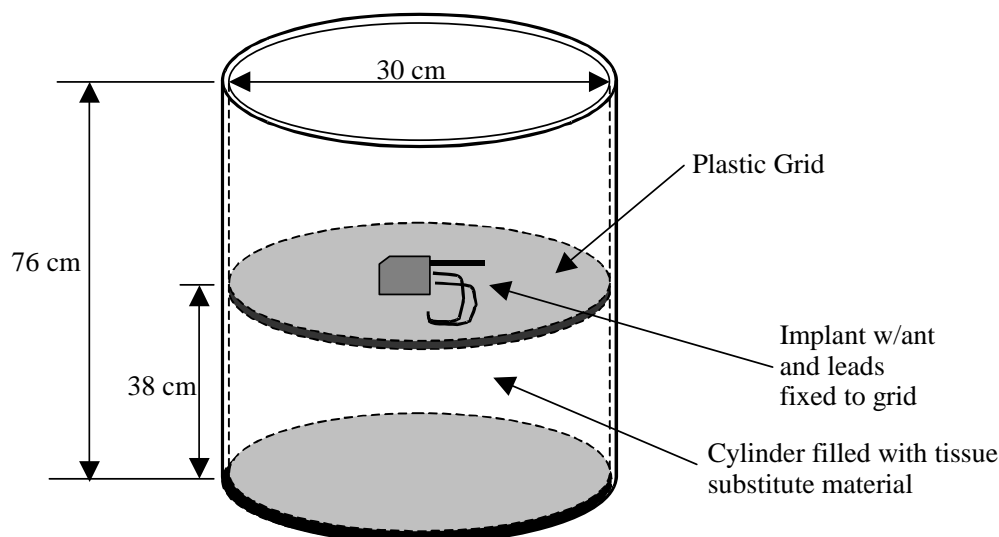
Figure B.1: Test fixture
