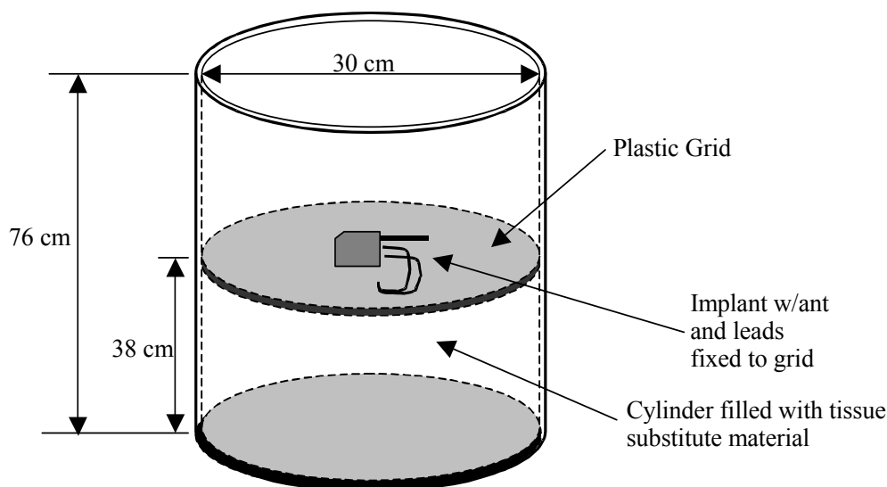
Figure C.1: Test fixture
