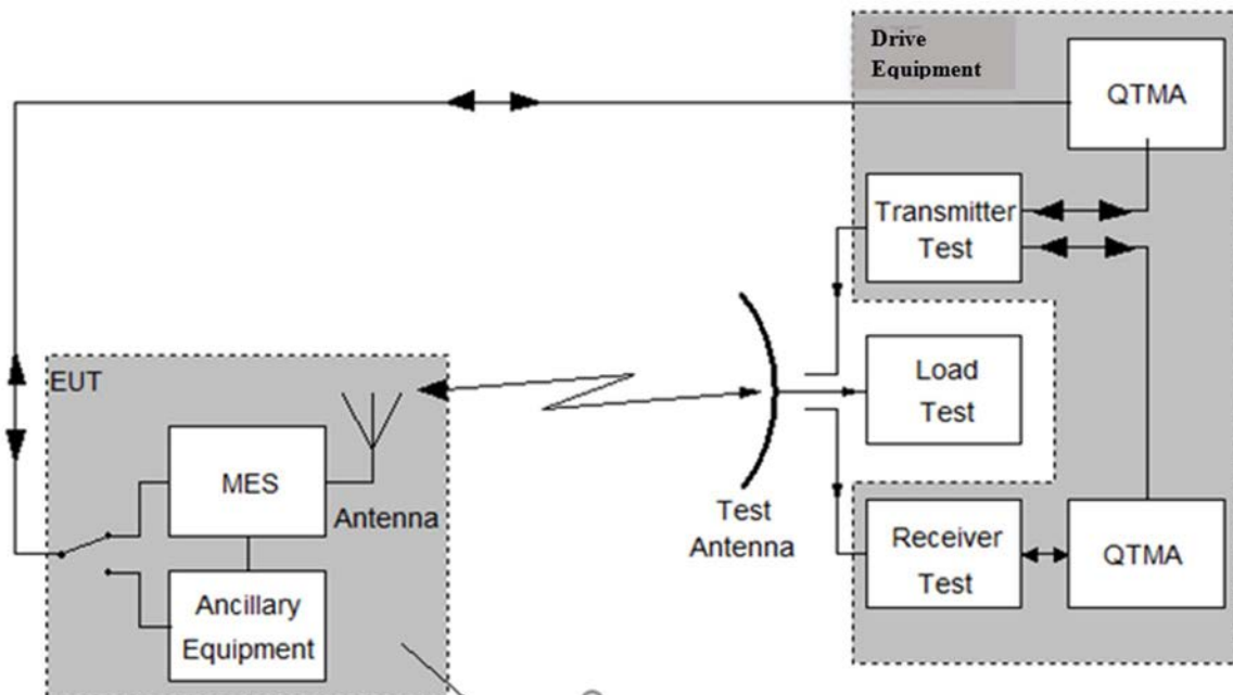
Figure 1: Test configuration
