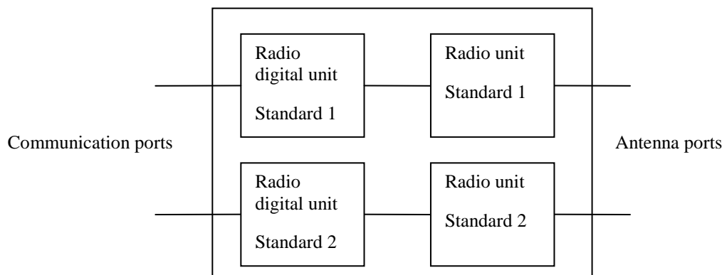
Figure 1: Multi-radio equipment
