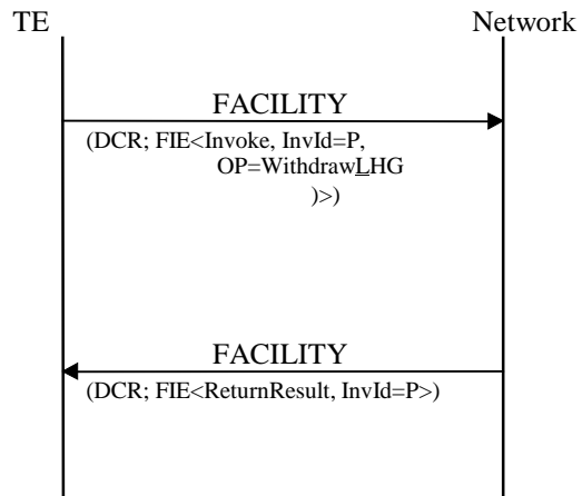
Figure A.1: Successful temporary withdrawal of an access from a hunt group
