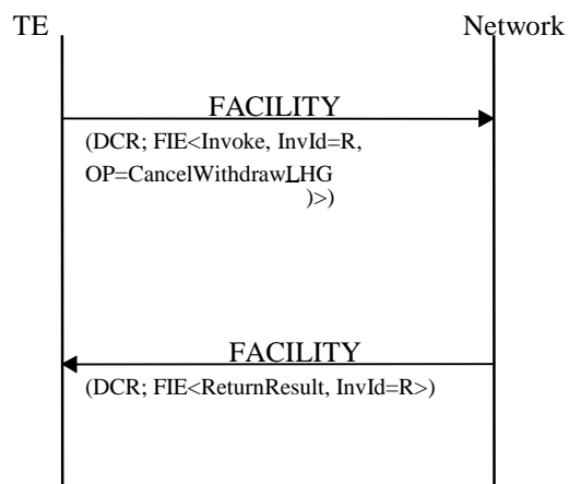
Figure A.2: Successful cancellation of withdrawal of an access from a hunt group
