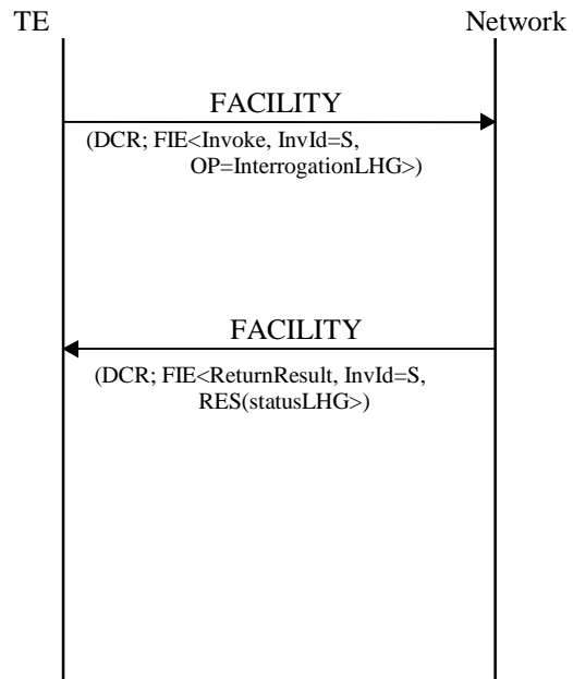
Figure A.3: Successful Interrogation of LHG
