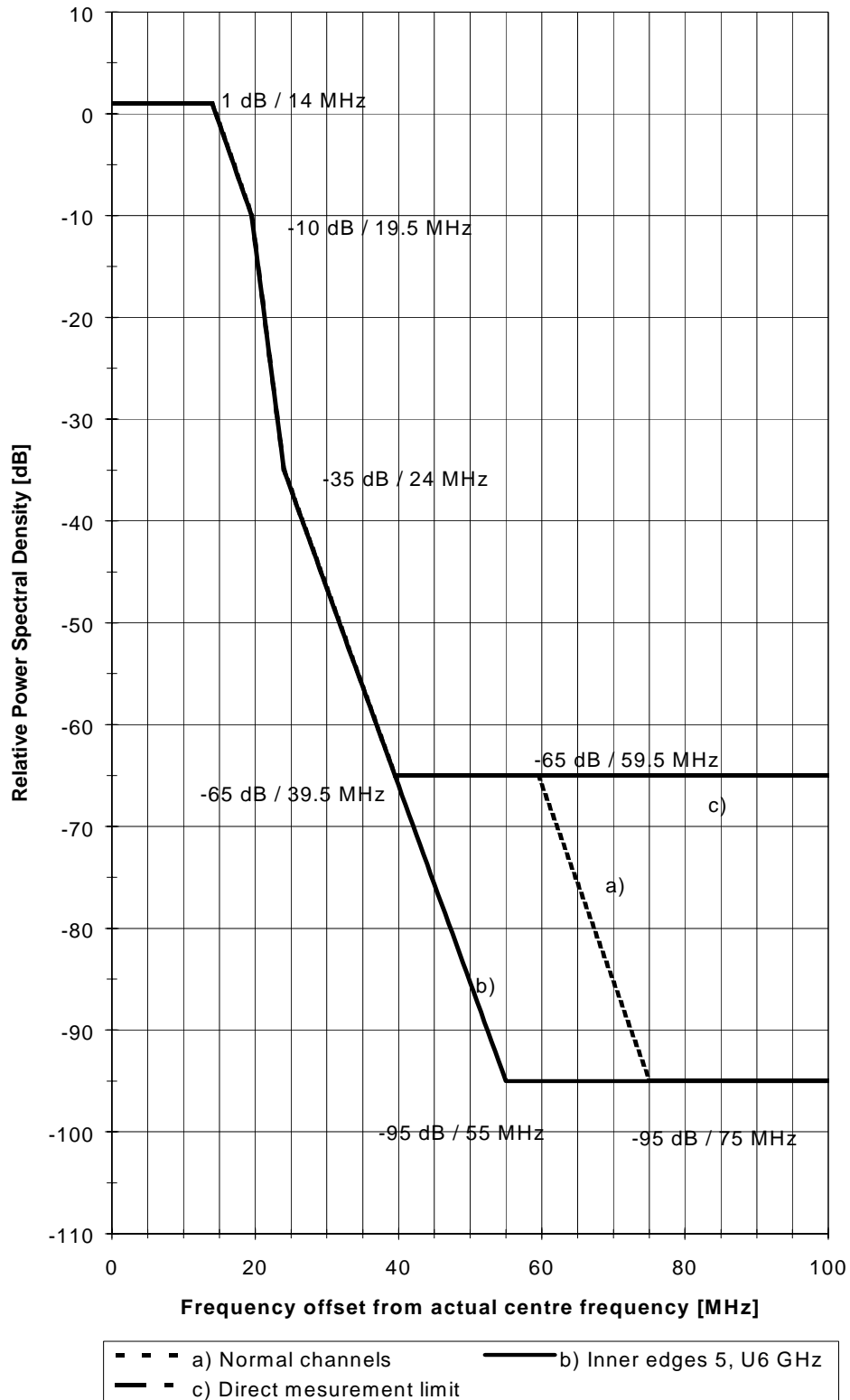
Figure 2: Limits of power spectral density
