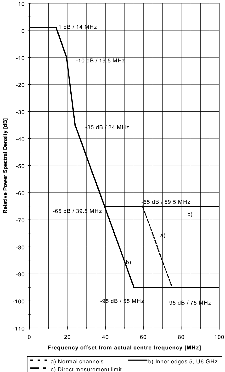
Figure 2: Limits of power spectral density
