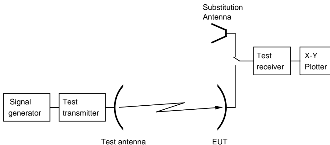
Figure 10: Test arrangement - antenna transmit gain measurement
