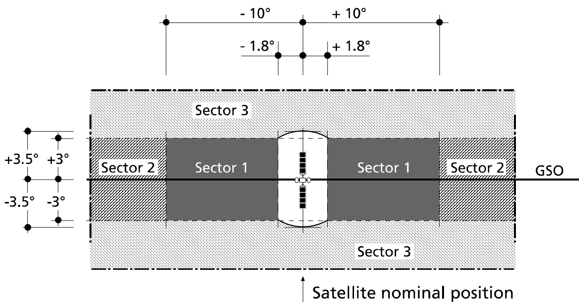
Figure 3: Different sectors for off-axis EIRP limits
