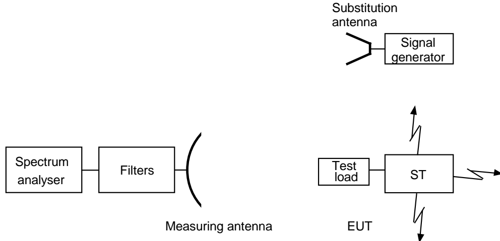
Figure 6: Test arrangement - spurious radiation measurements above 1 000 MHz for an EUT without antenna
