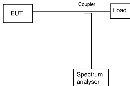
Figure 9: Test arrangement - transmit output power density measurement
