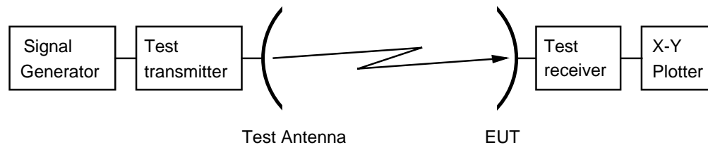
Figure 11: Test arrangement - antenna transmit radiation pattern measurement
