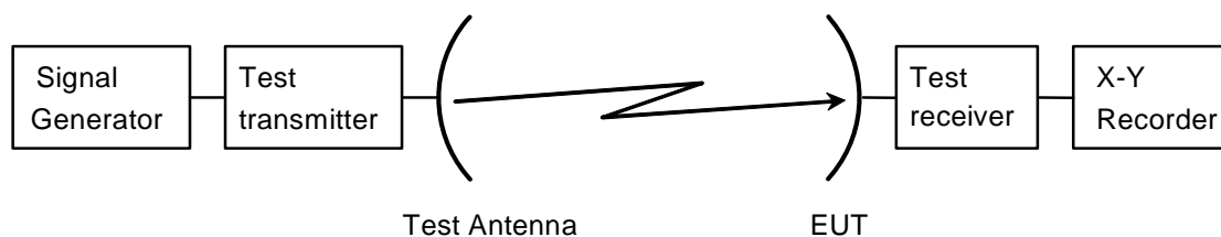
Figure 9: Test arrangement-antenna transmit radiation pattern measurement
