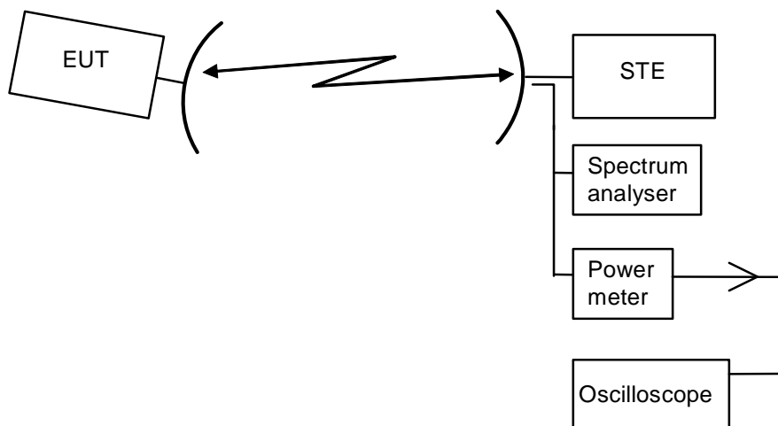
Figure 10: Test arrangement for pointing error detection
